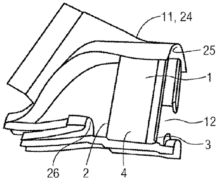
PRIOR ART
