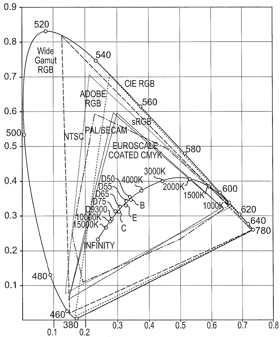
CIE 1931 NORMALIZED TABLE
