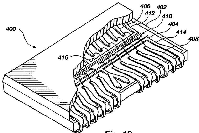
Fig. 18 (PRIOR ART)
