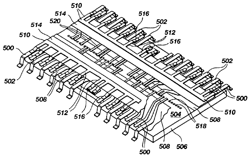
Fig. 19 (PRIOR ART)
