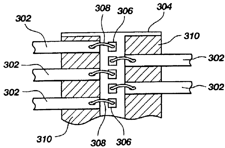
Fig. 17 (PRIOR ART)
