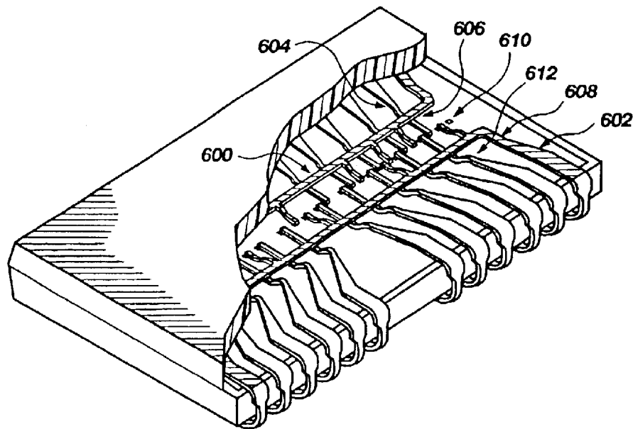
Fig. 20 (PRIOR ART)
