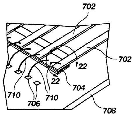
Fig. 21 (PRIOR ART)
