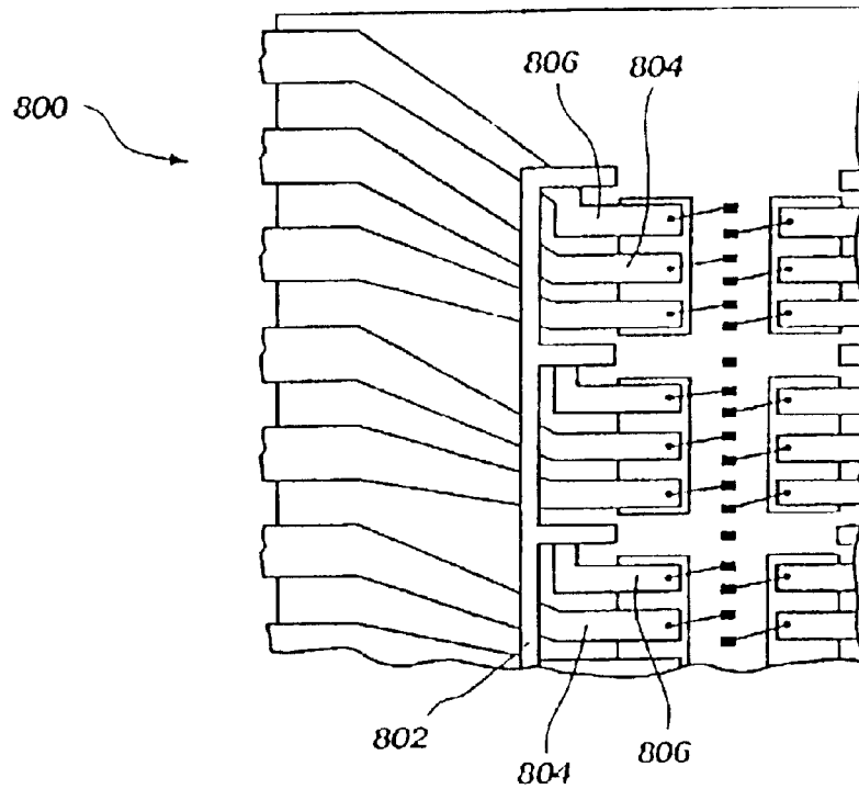
Fig. 23 (PRIOR ART)
