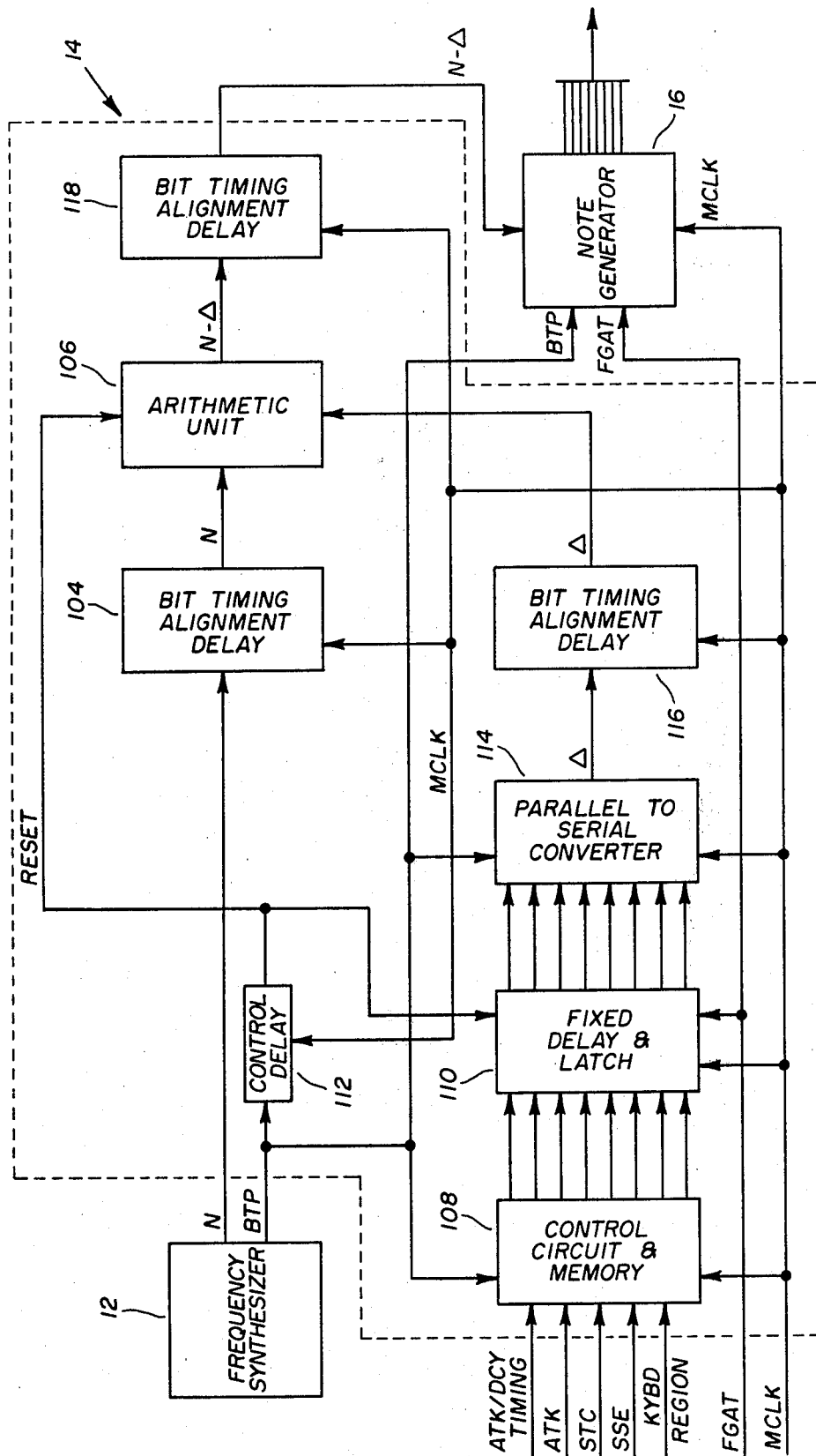
PITCH SHIFTER CONTROL FIG. 2
