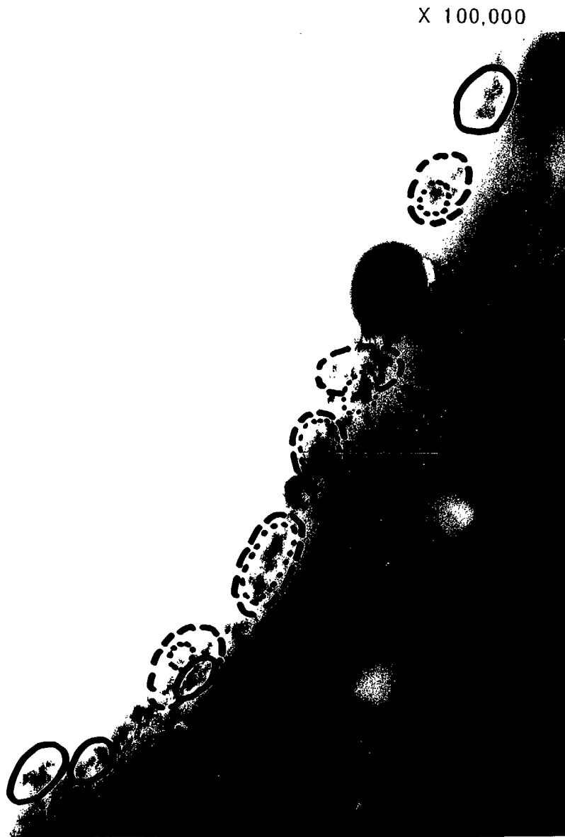
Electron micrograph of a cut surface of toner of Comparative Example 10 (Small- and large-particle negatively chargeable silicas + Titania + Small-particle positively chargeable silica)
