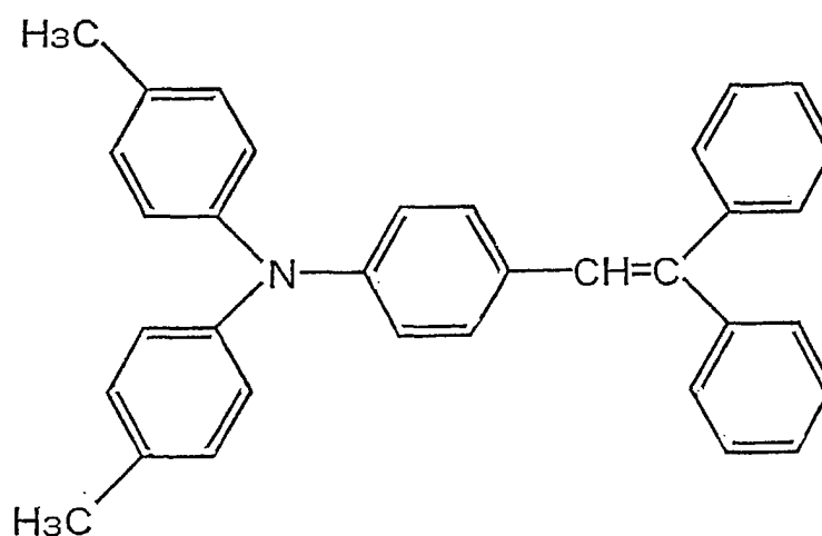
Structural Formula (1)
