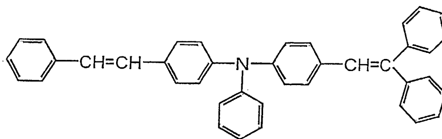
Structural Formula (2)
