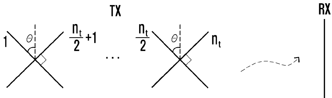
(a) Rotated dual-polarized MISO scenario
