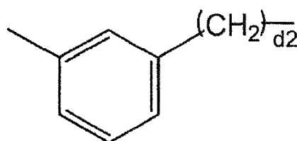
[Chemical Formula 8]
