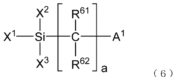
[Chemical Formula 1]
