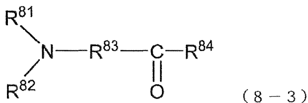
[Chemical Formula 20]
