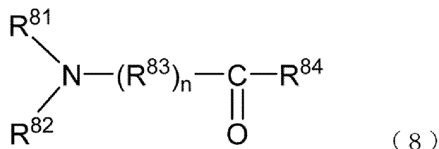
[Chemical Formula 3]
