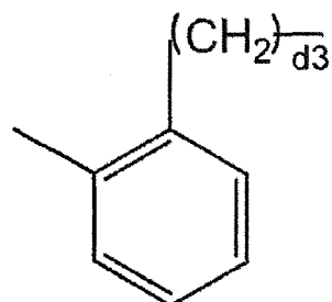
[Chemical Formula 8]
