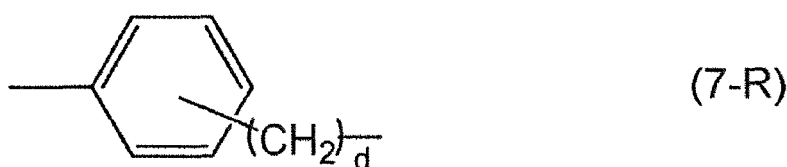
[Chemical Formula 5]
