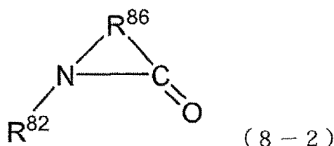
[Chemical Formula 19]
