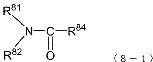
[Chemical Formula 18]
