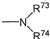
[Chemical Formula 9]
