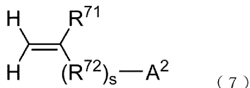
[Chemical Formula 2]
