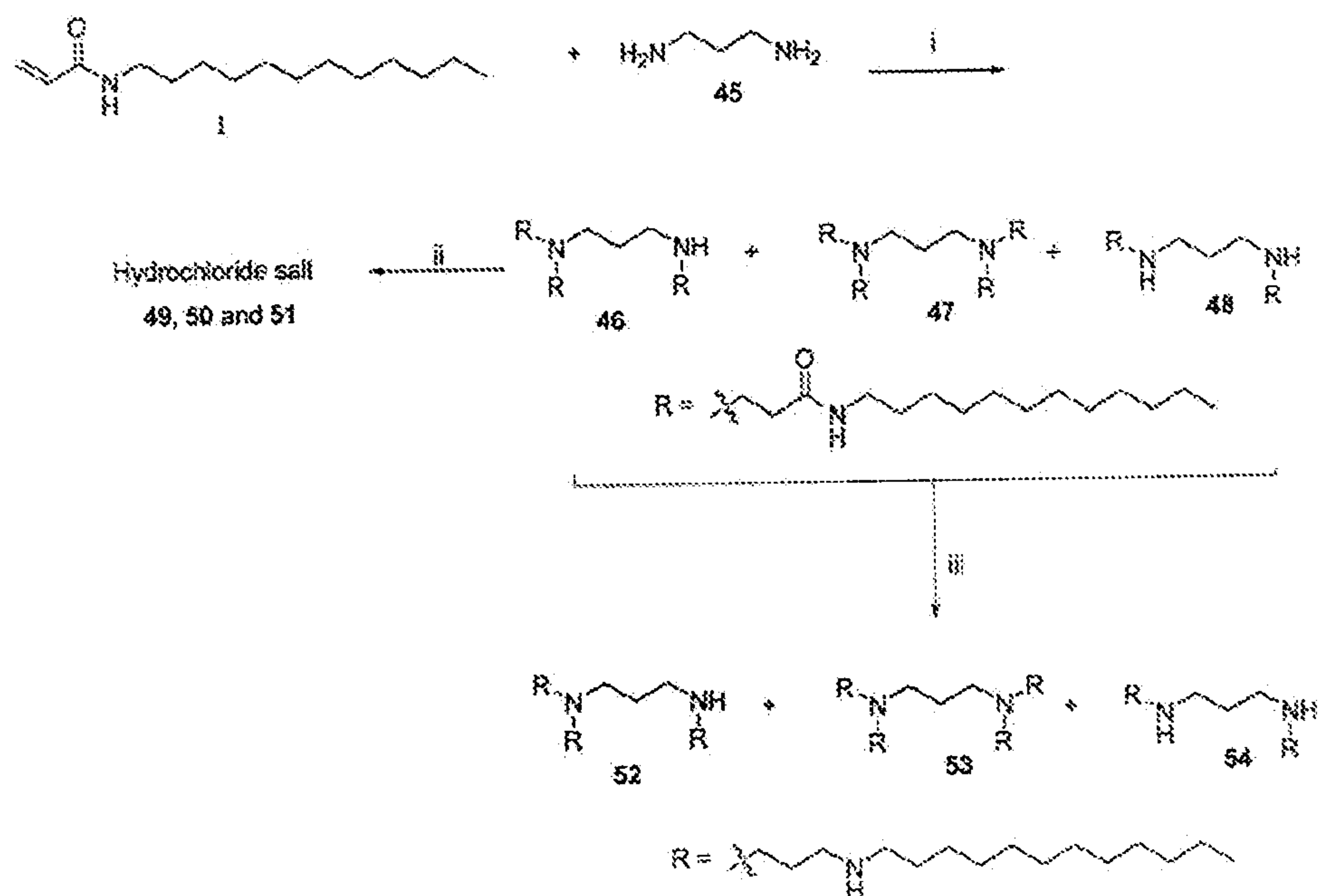
Scheme 18 a
