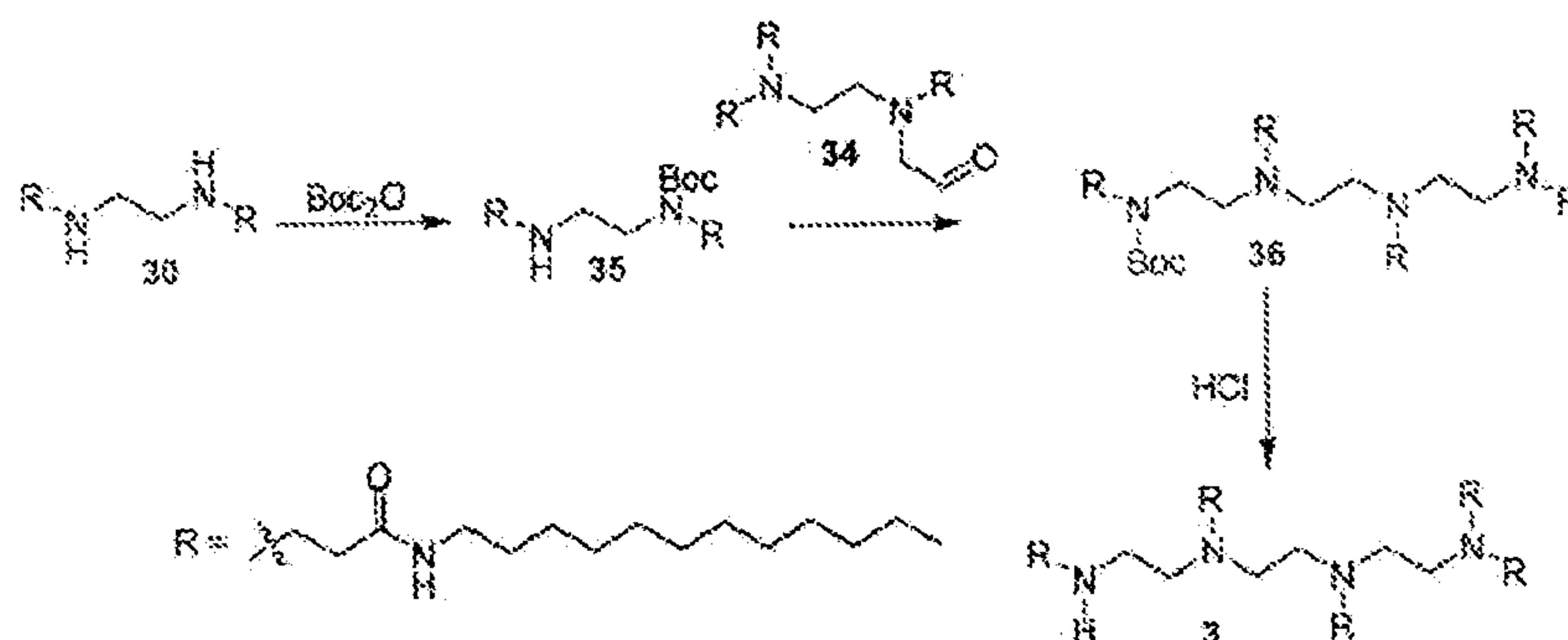
Scheme 15
