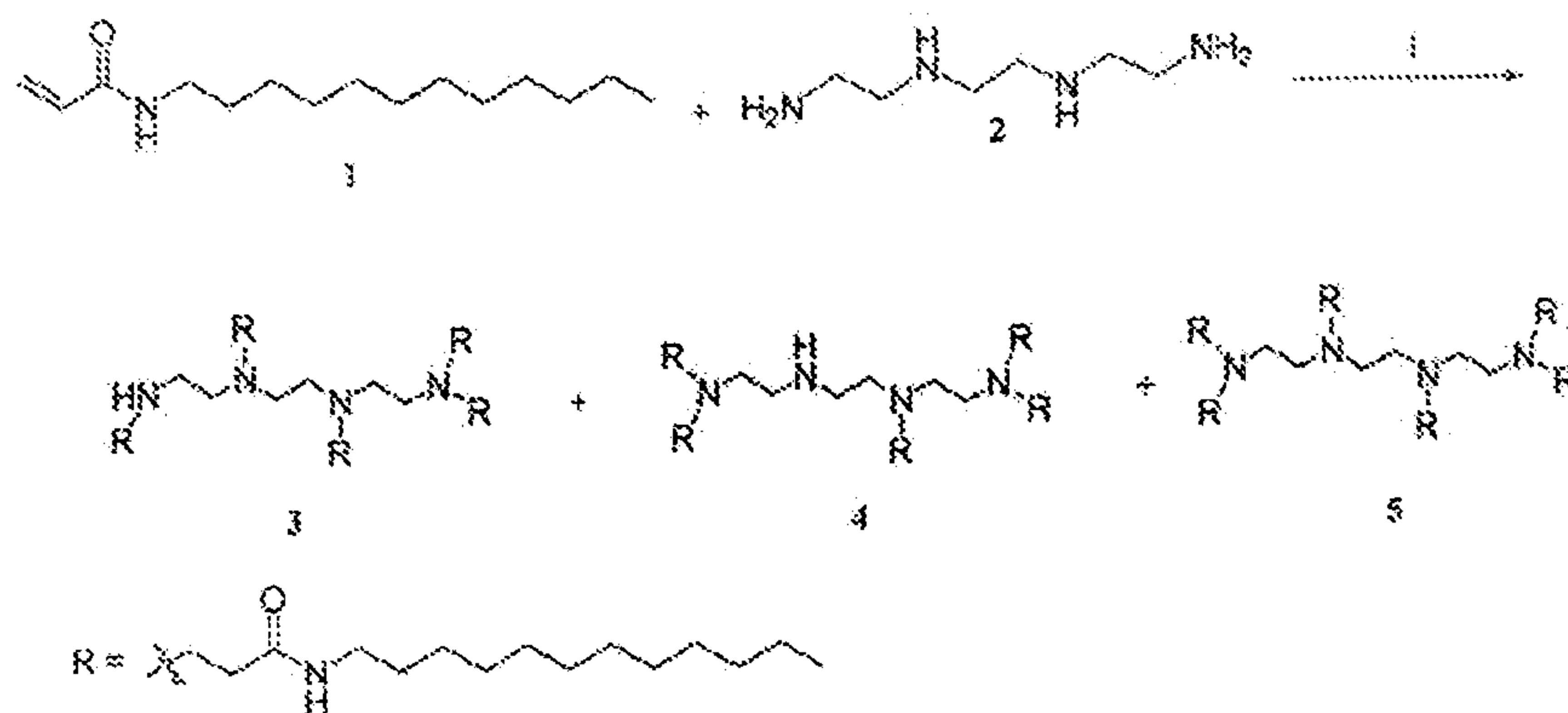
Scheme 1 a
