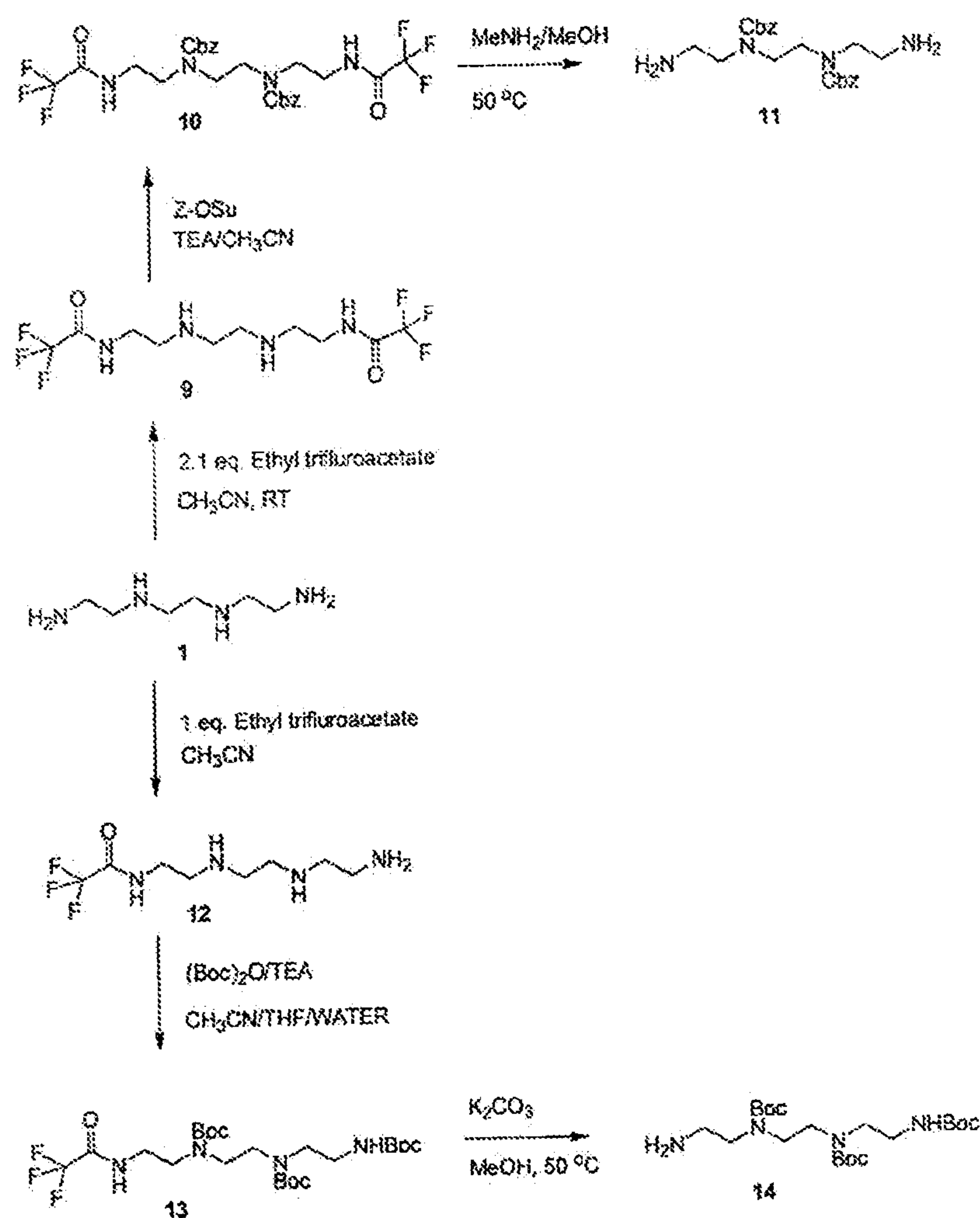
Scheme 8 a
