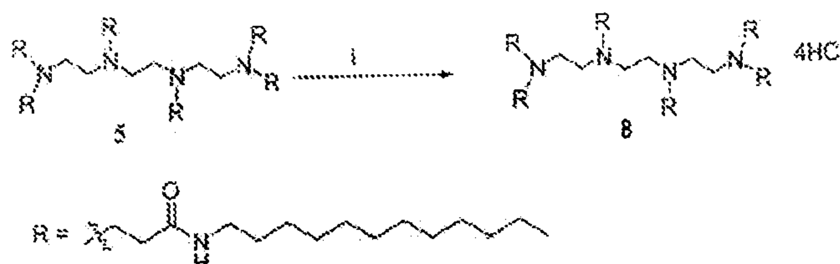
Scheme 7 a
