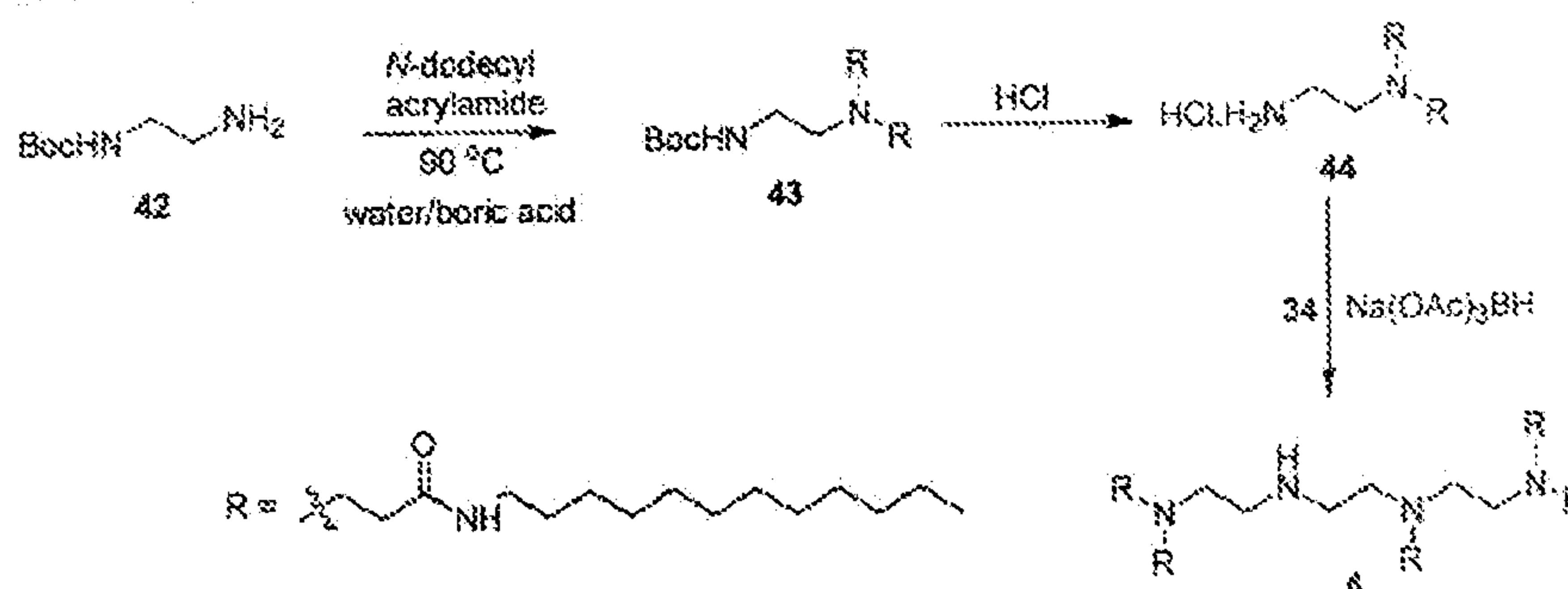
Scheme 17
