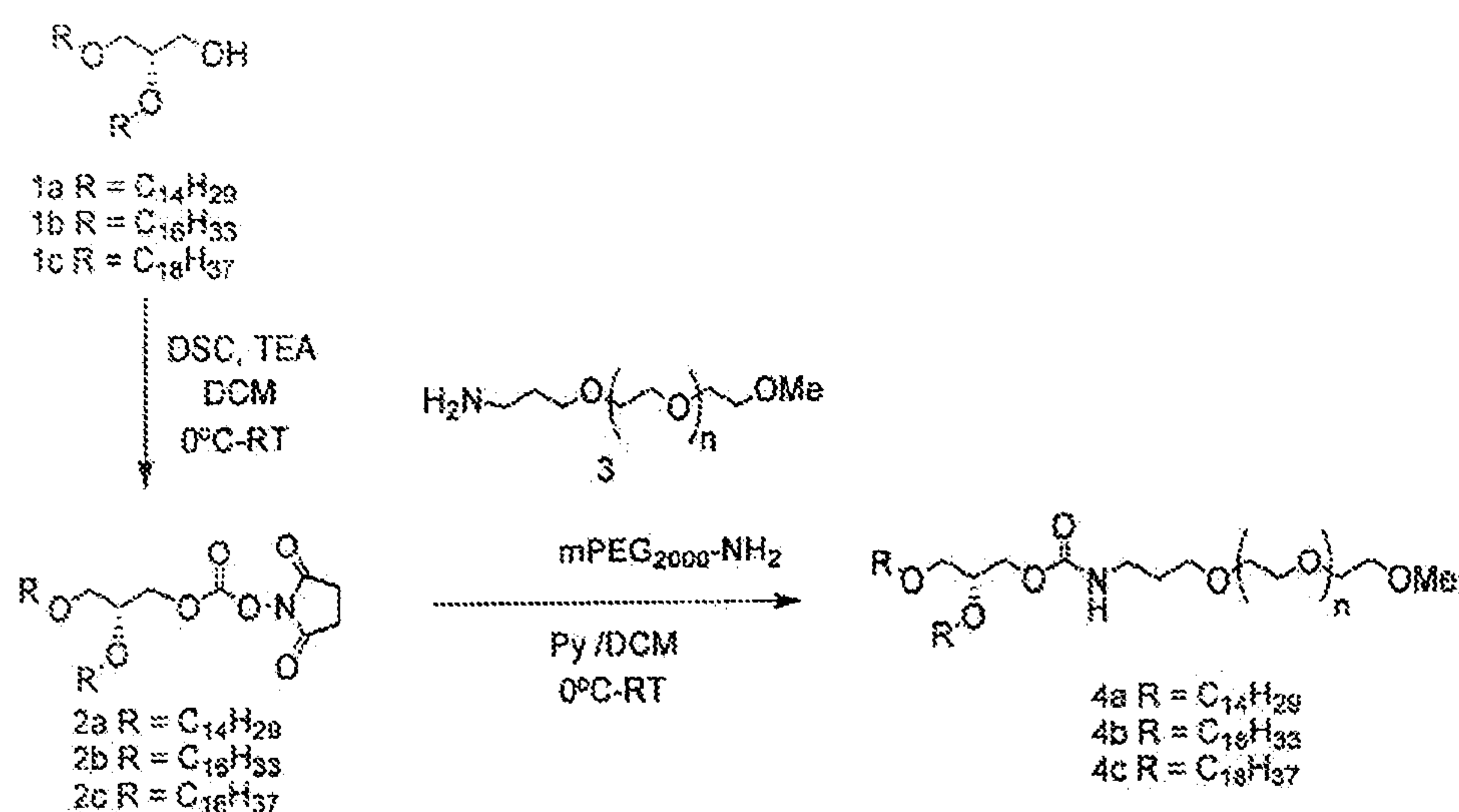
Scheme 1 a
