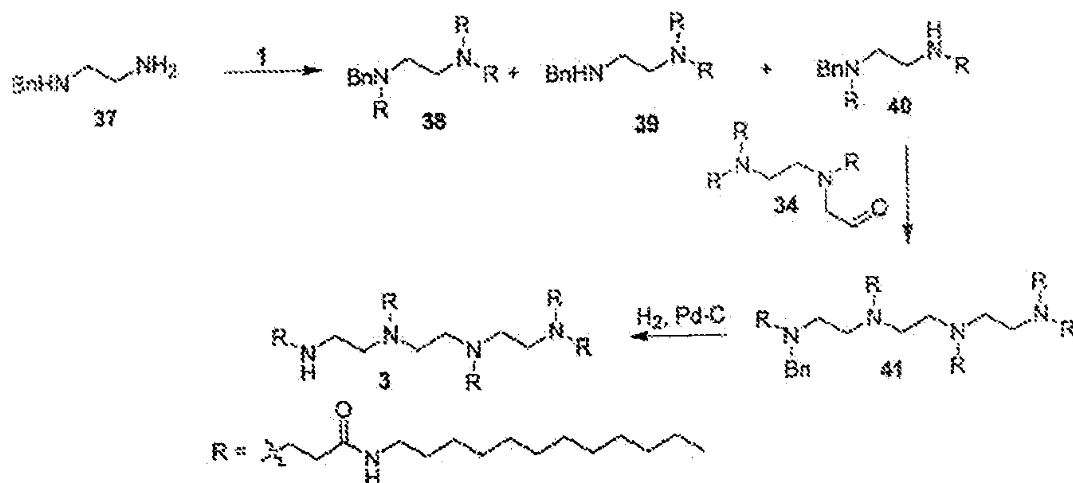
Scheme 16
