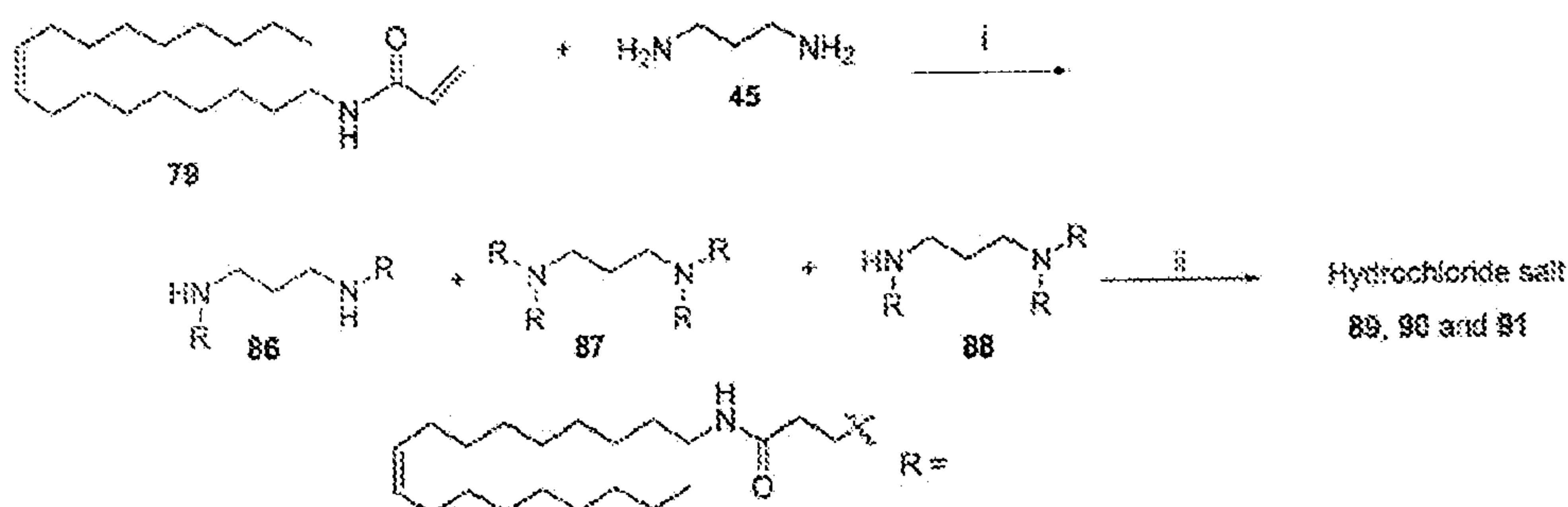
Scheme 25 a
