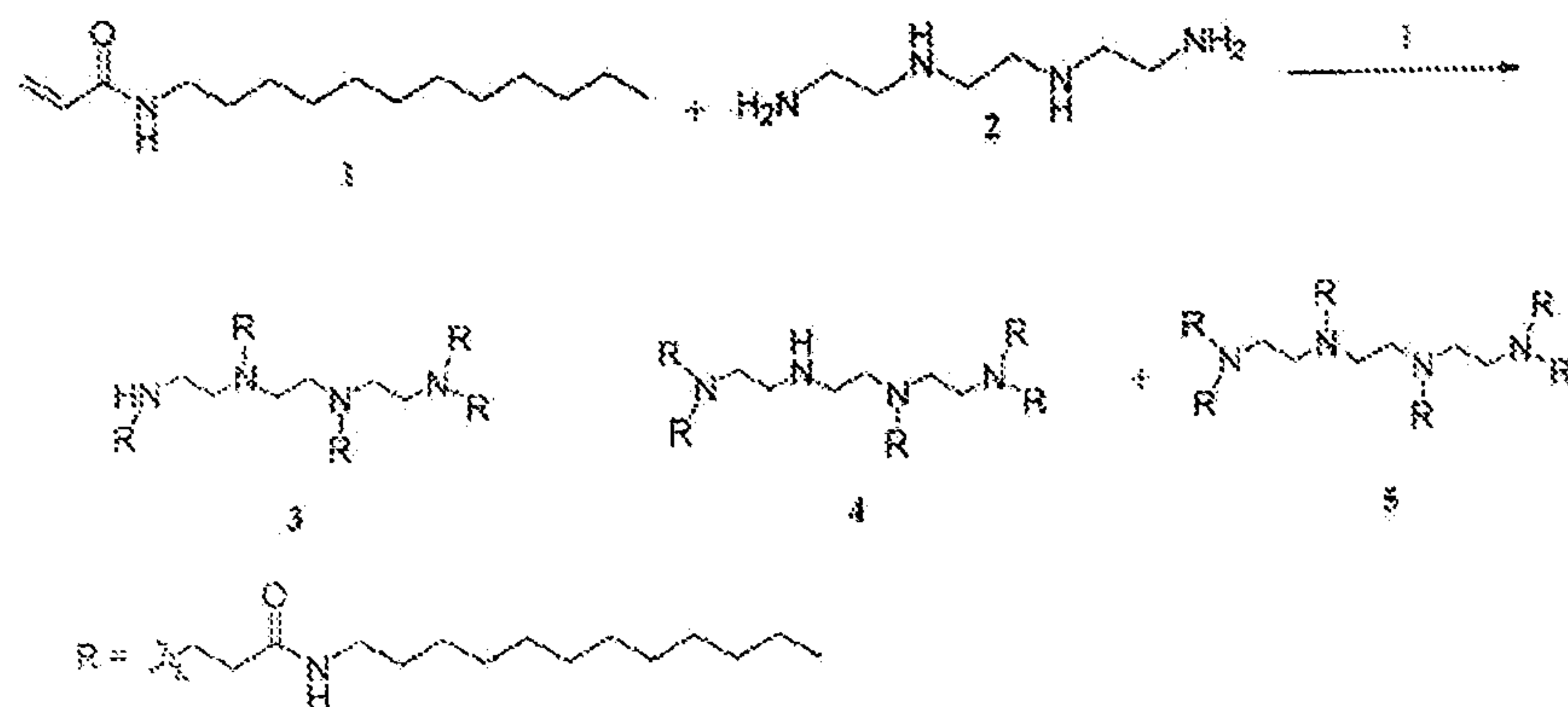
Scheme 3 a
