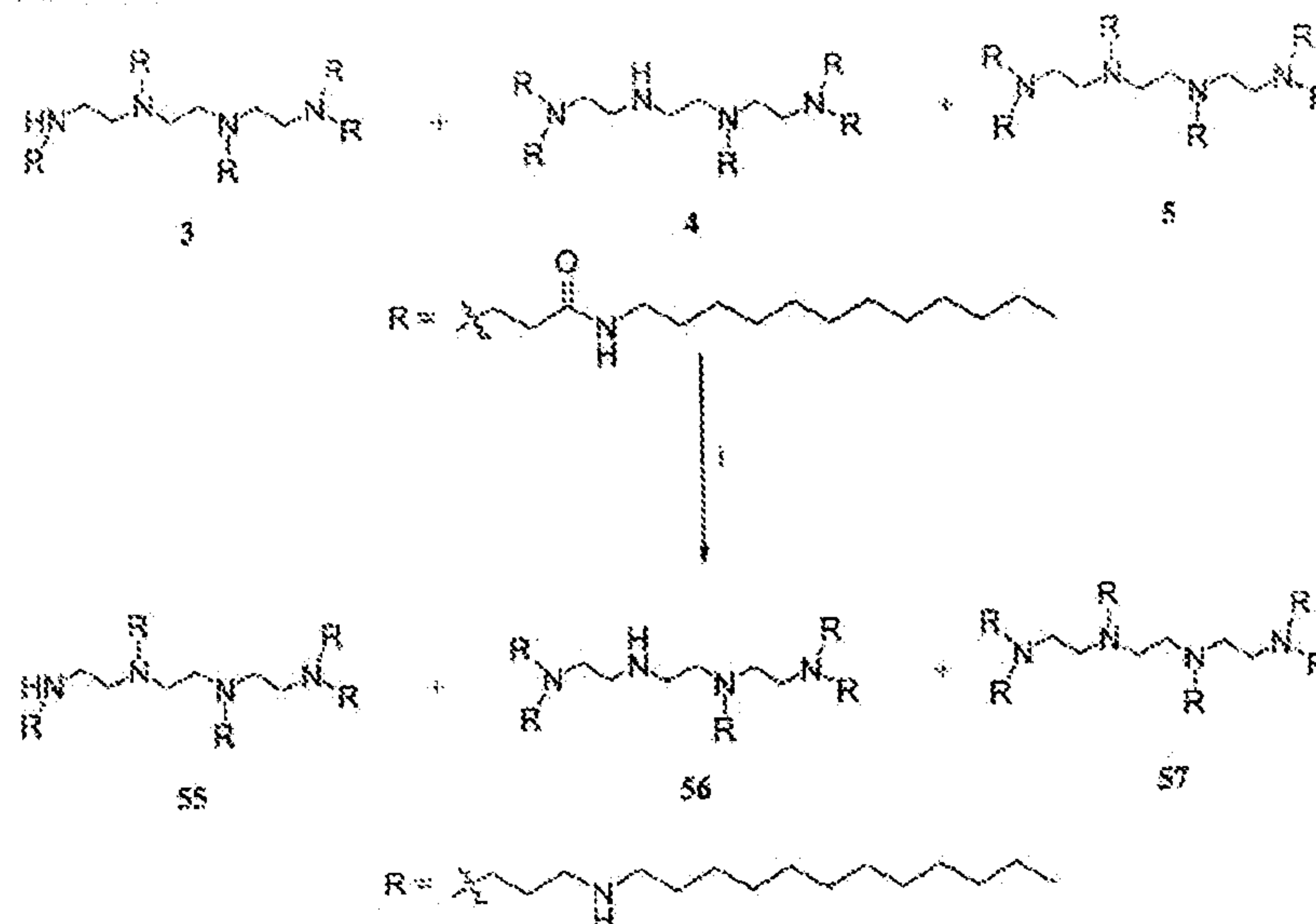
Scheme 19 b
