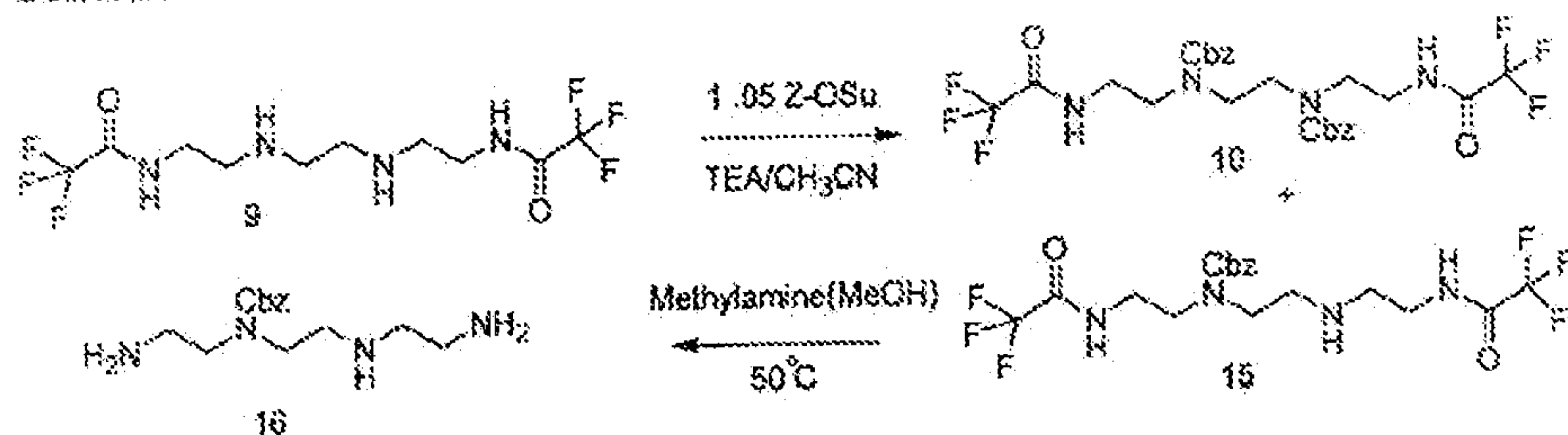
Scheme 9 a
