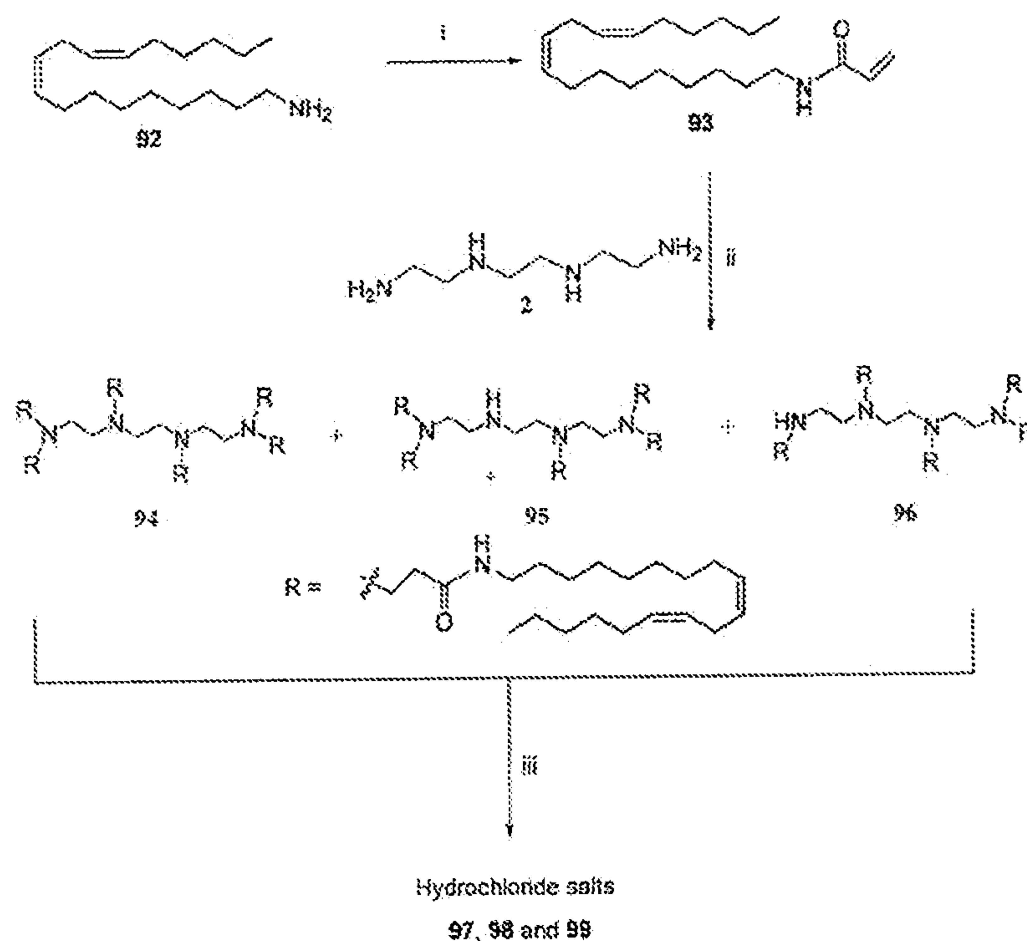
Scheme 26 a
