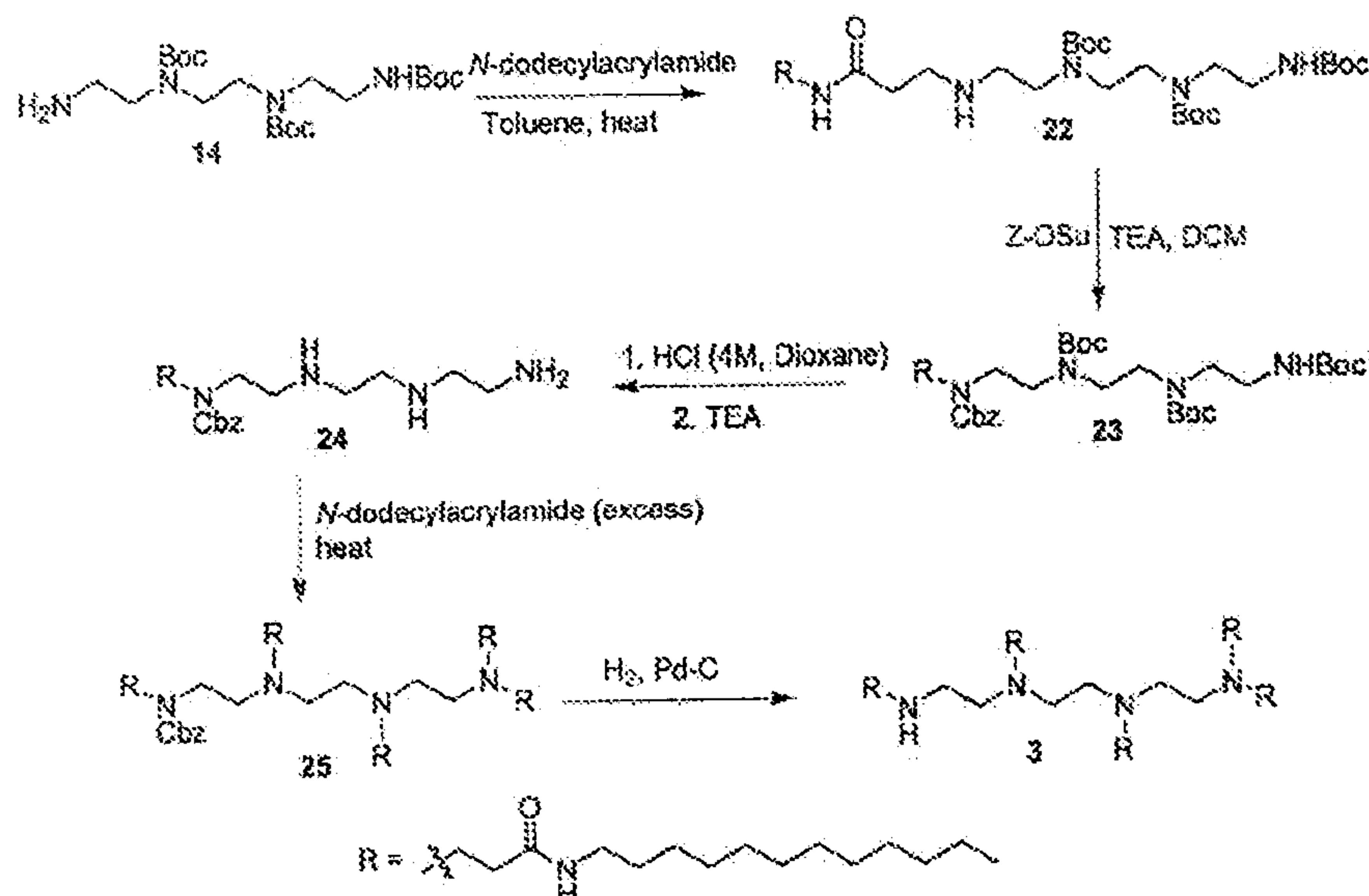
Scheme 12
