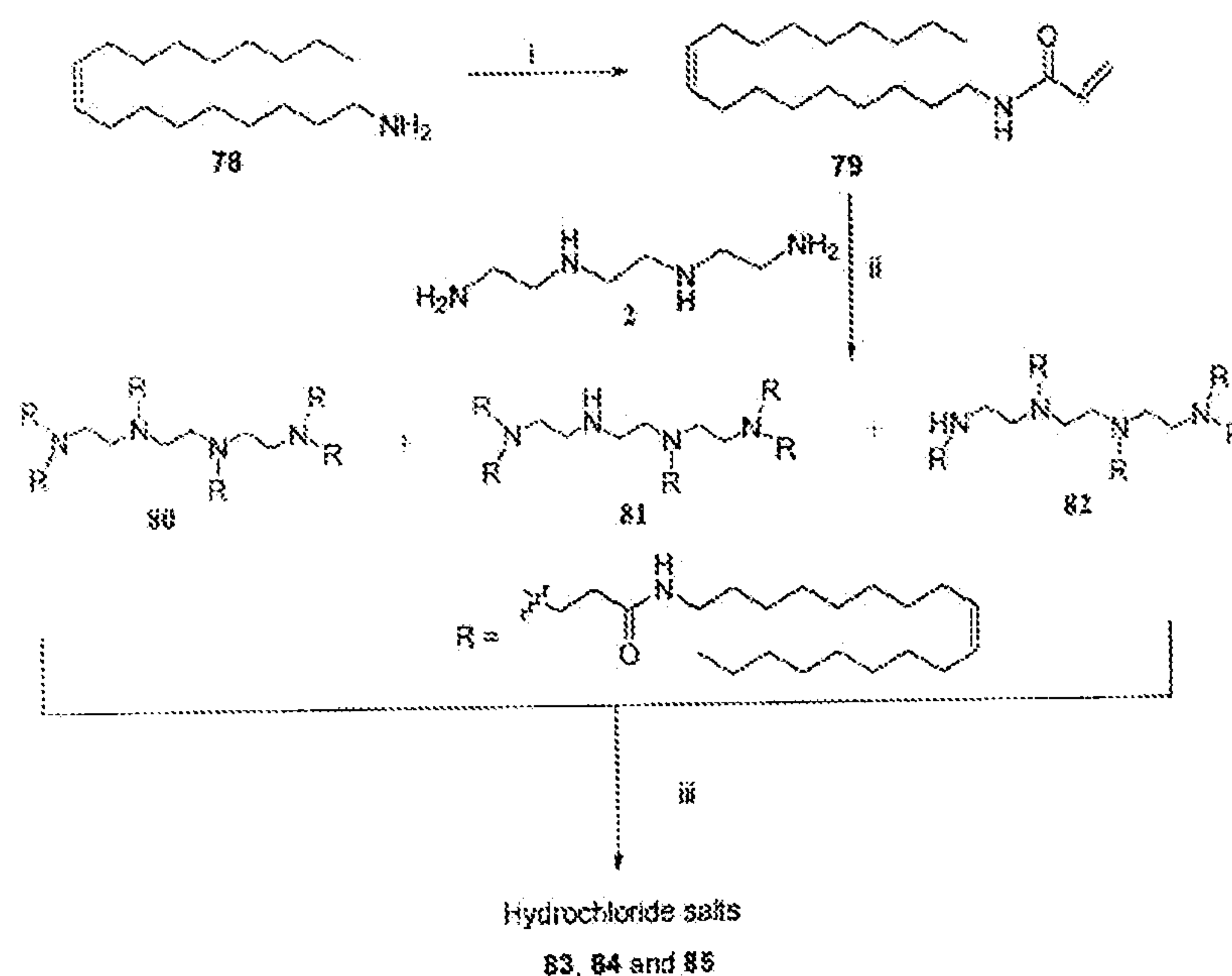
Scheme 24 a
