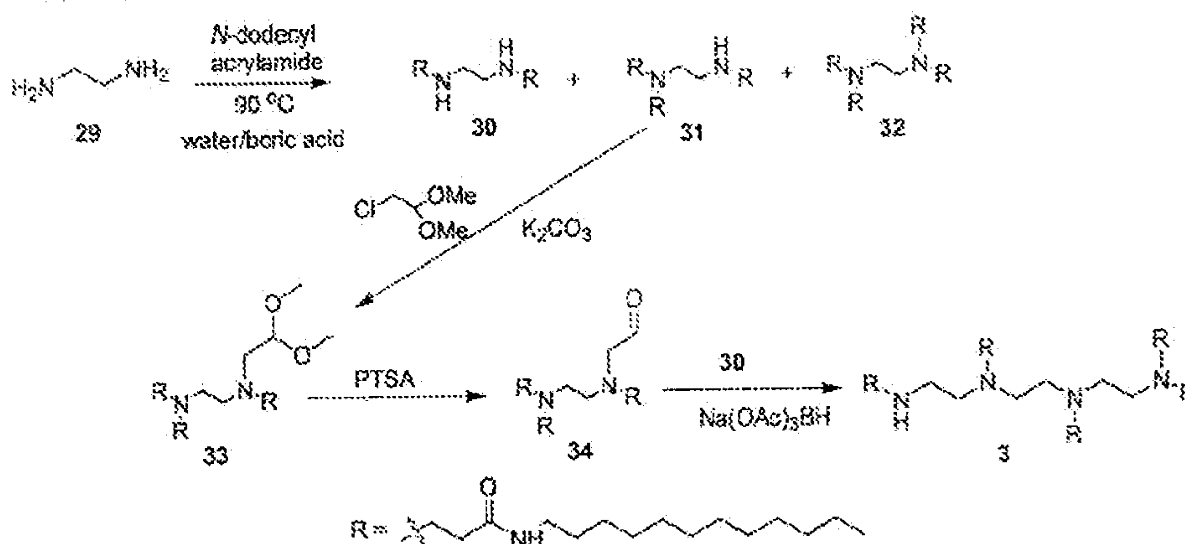
Scheme 8
