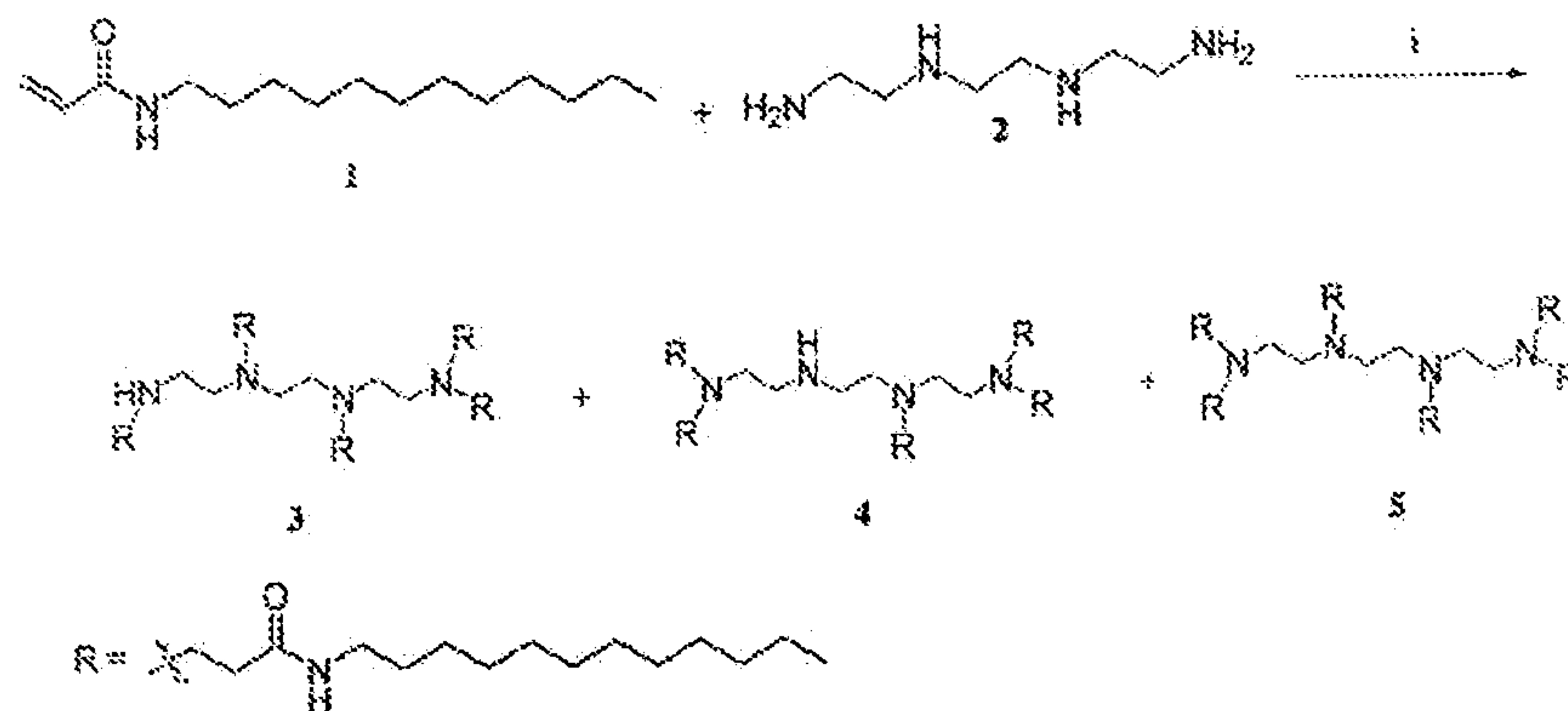
Scheme 2 a
