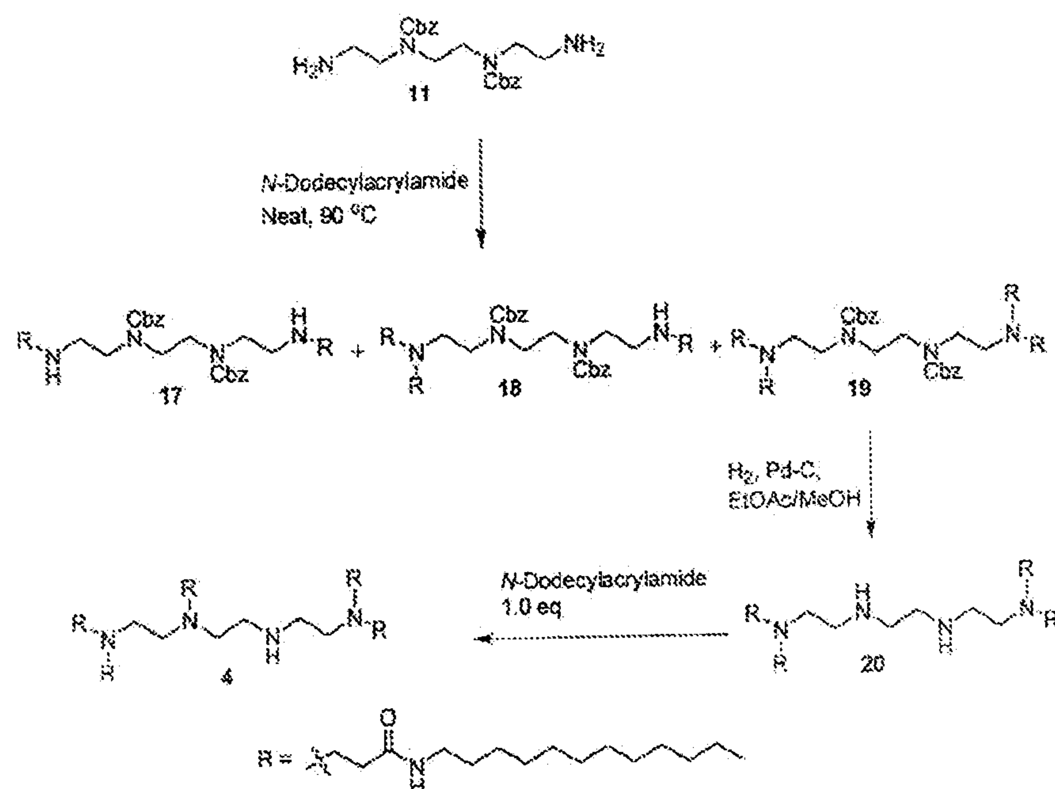
Scheme 10
