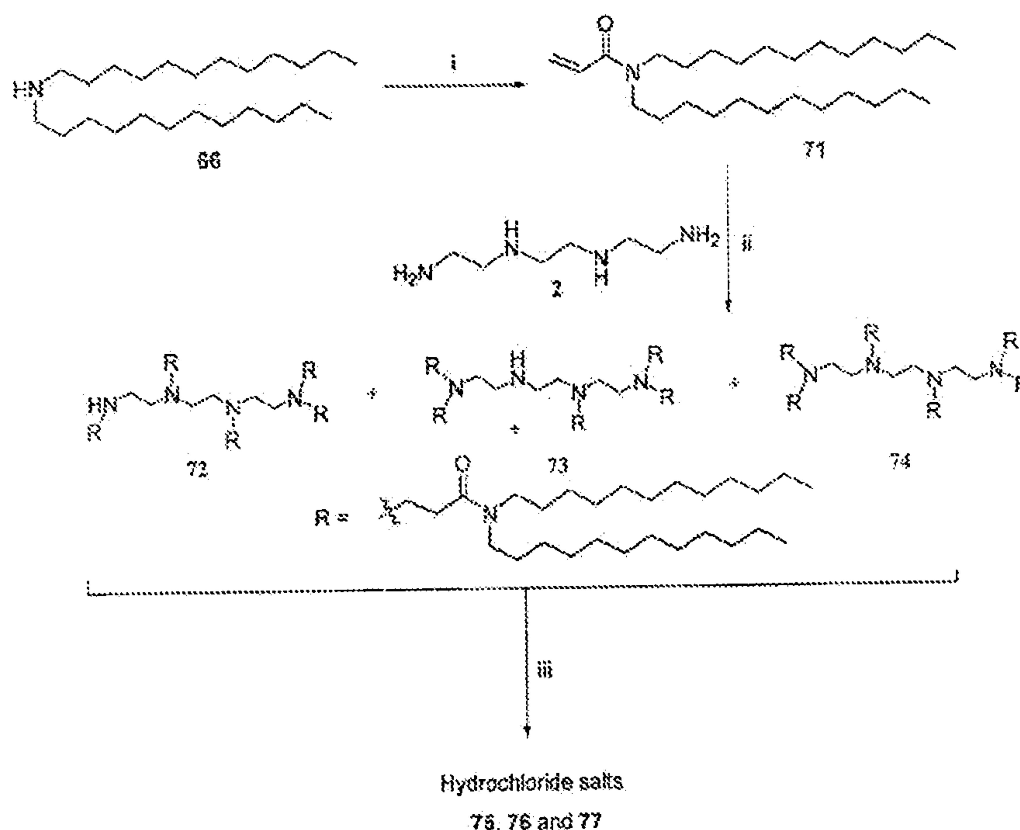
Scheme 23 a
