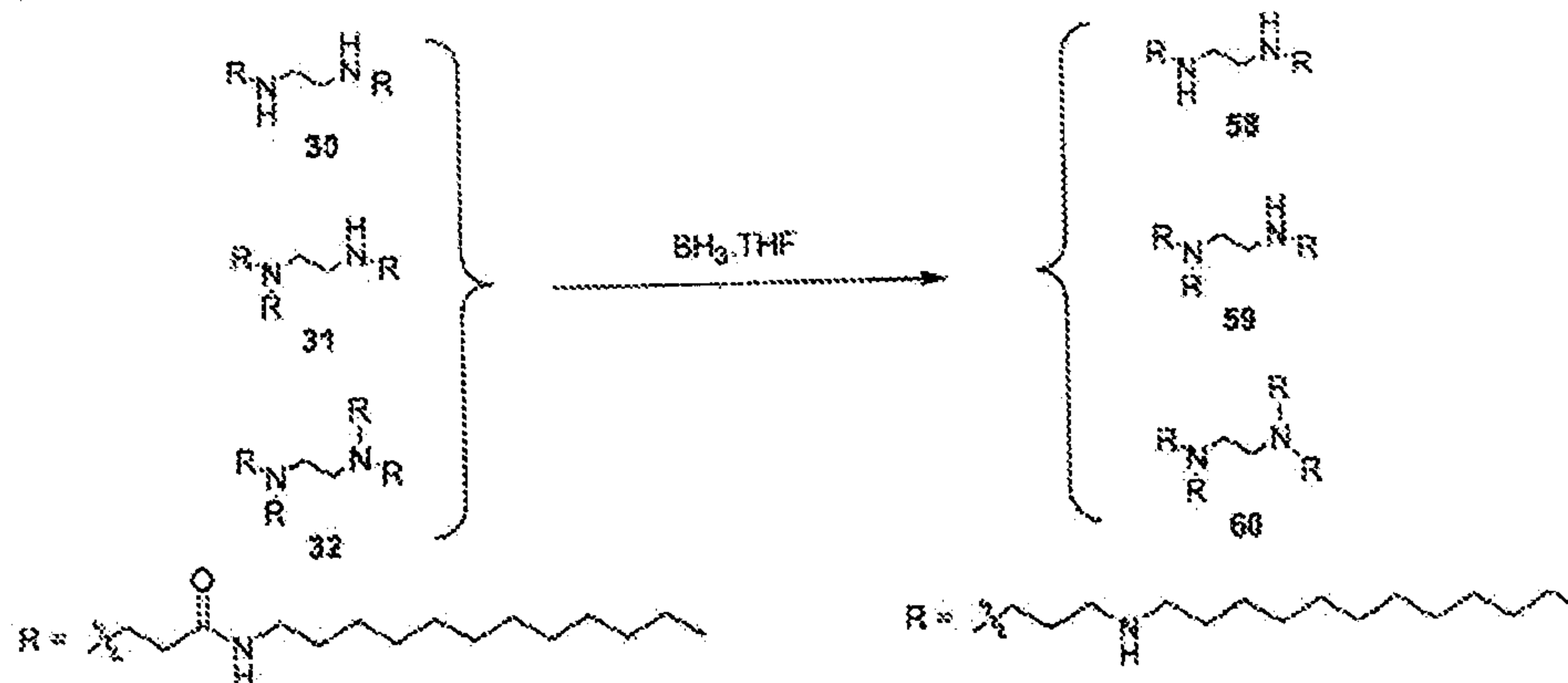
Scheme 20
