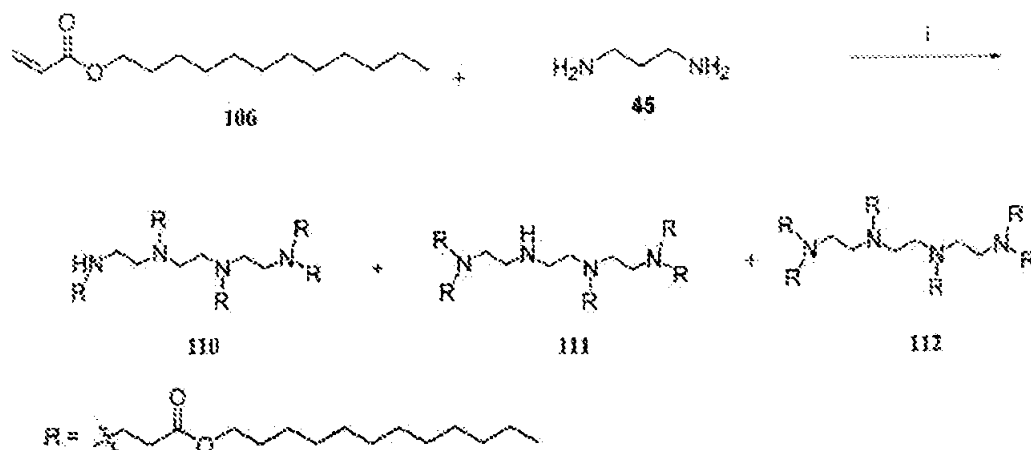
Scheme 29 a
