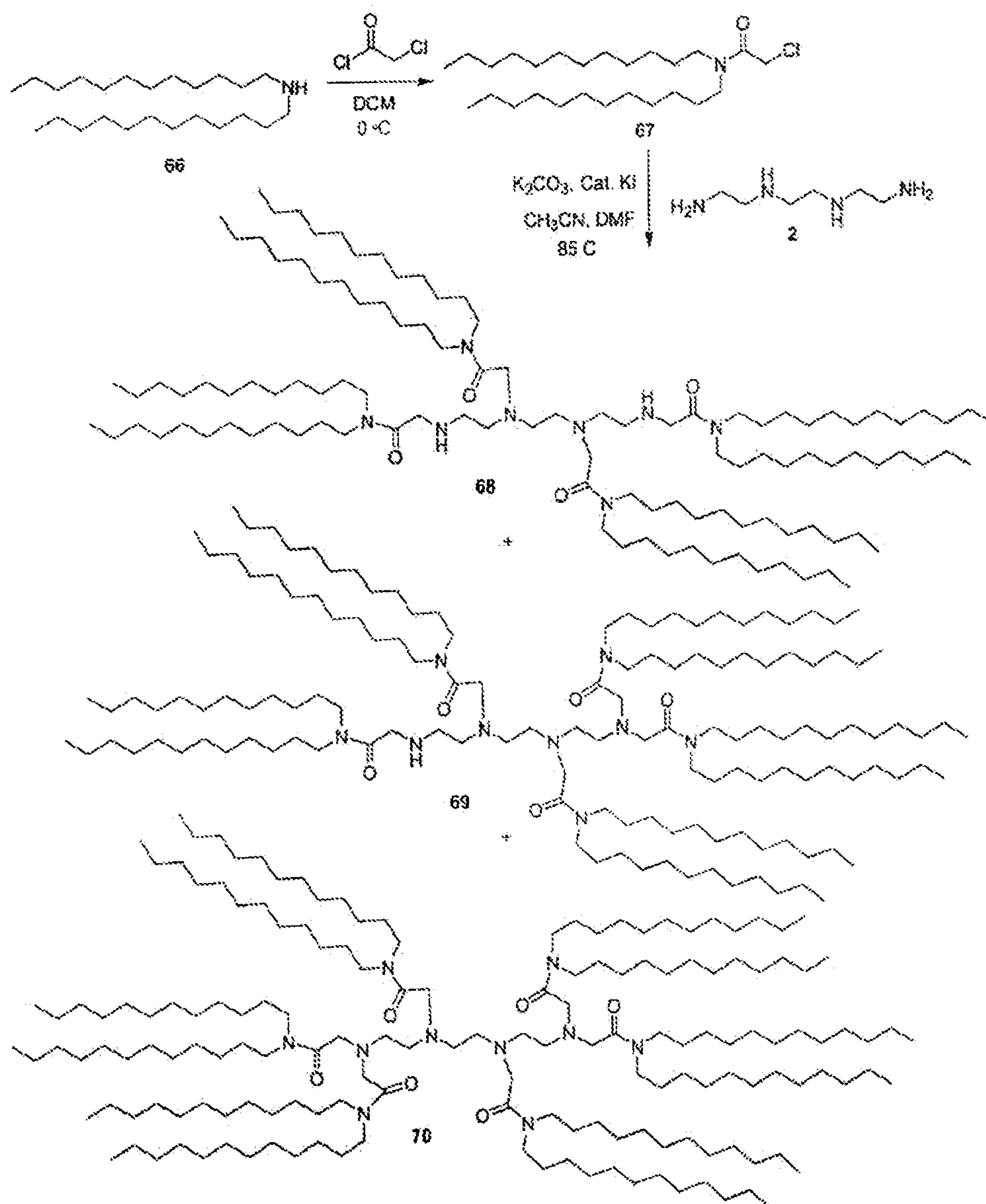
Scheme 22
