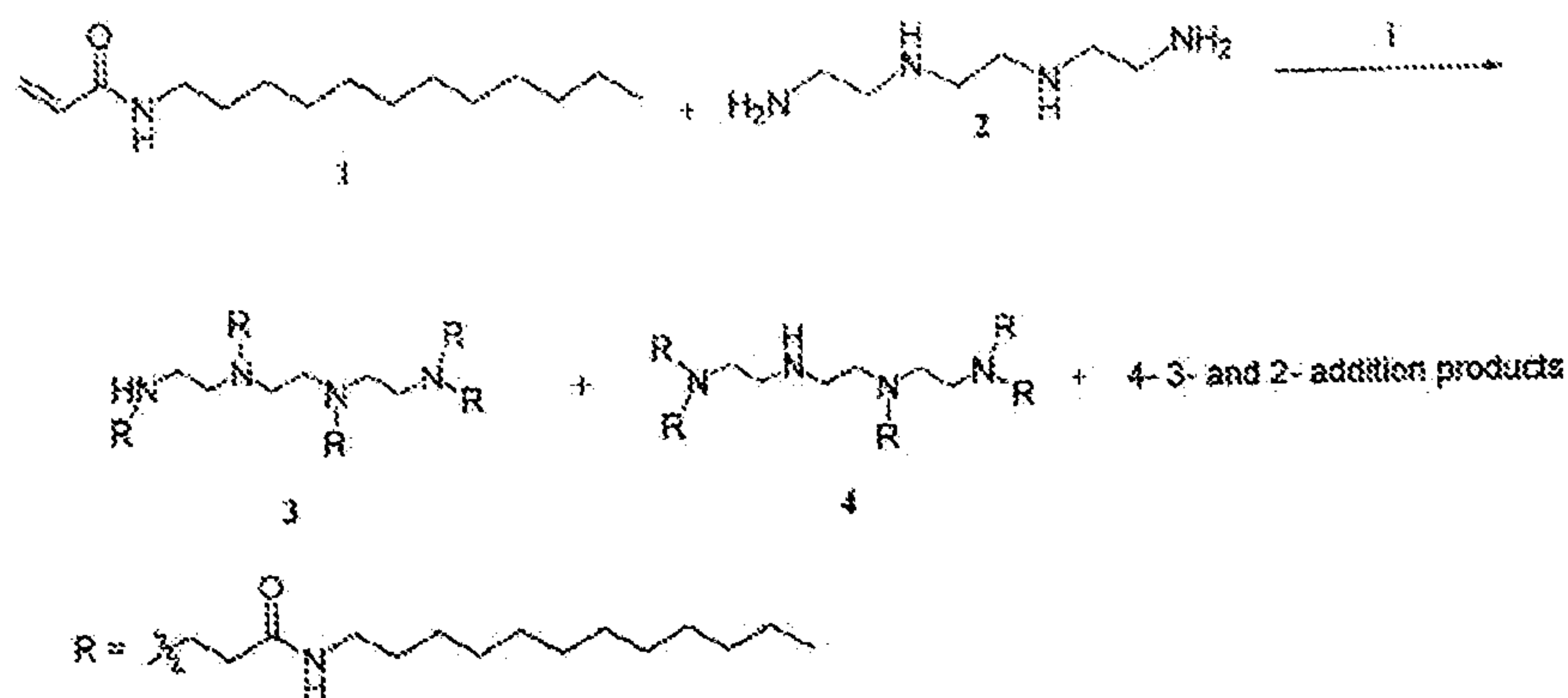
Scheme 4 a
