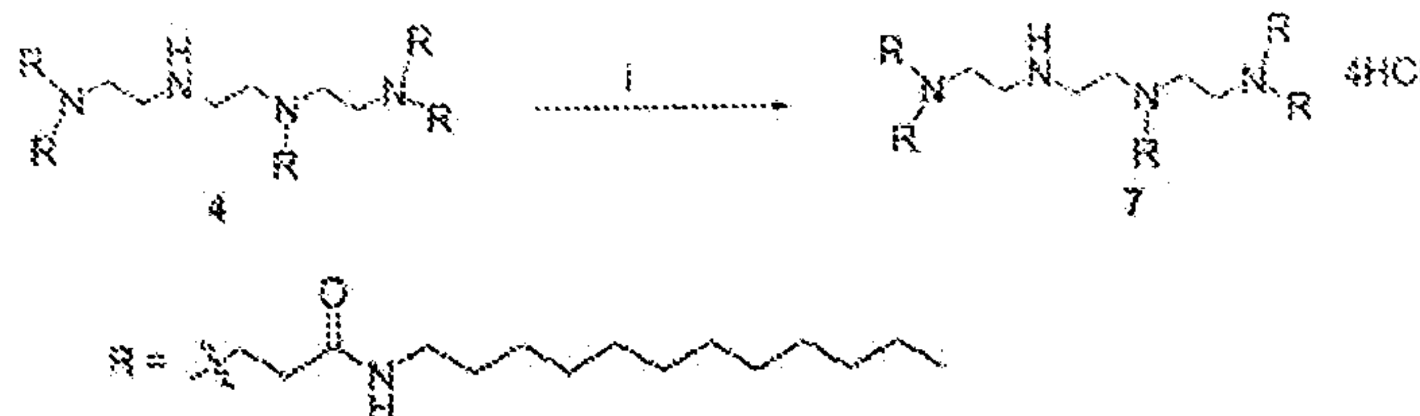
Scheme 6 a
