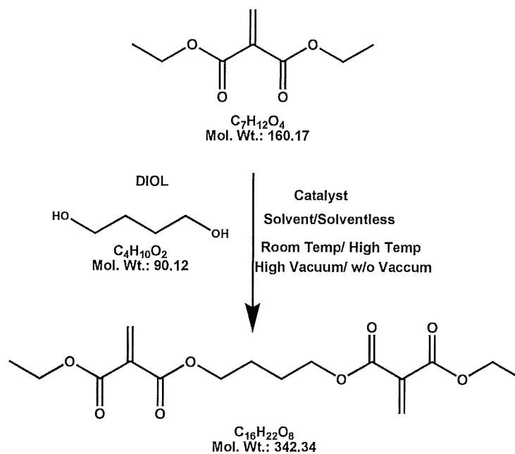
SCHEME 2A: Formation of MMM by Transesterification with diol
