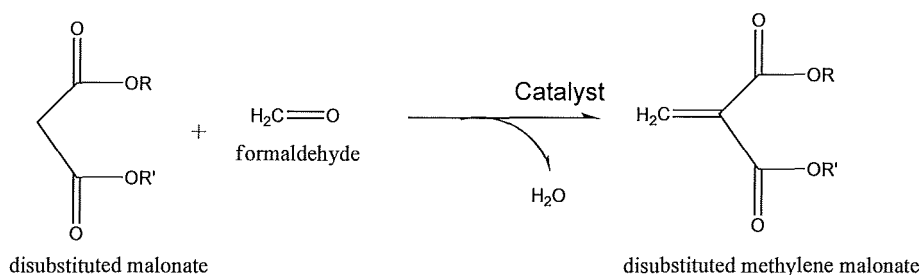
Schematic 1. Knoevenagel reaction with formaldehyde for the synthesis of a methylene malonate.
