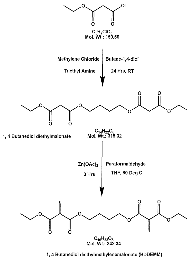
Scheme 1: Formation of MMM through modified Knoevenagel Reaction
