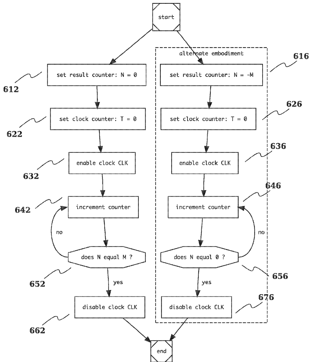
Fig. 7 Count-To-Time Mode
