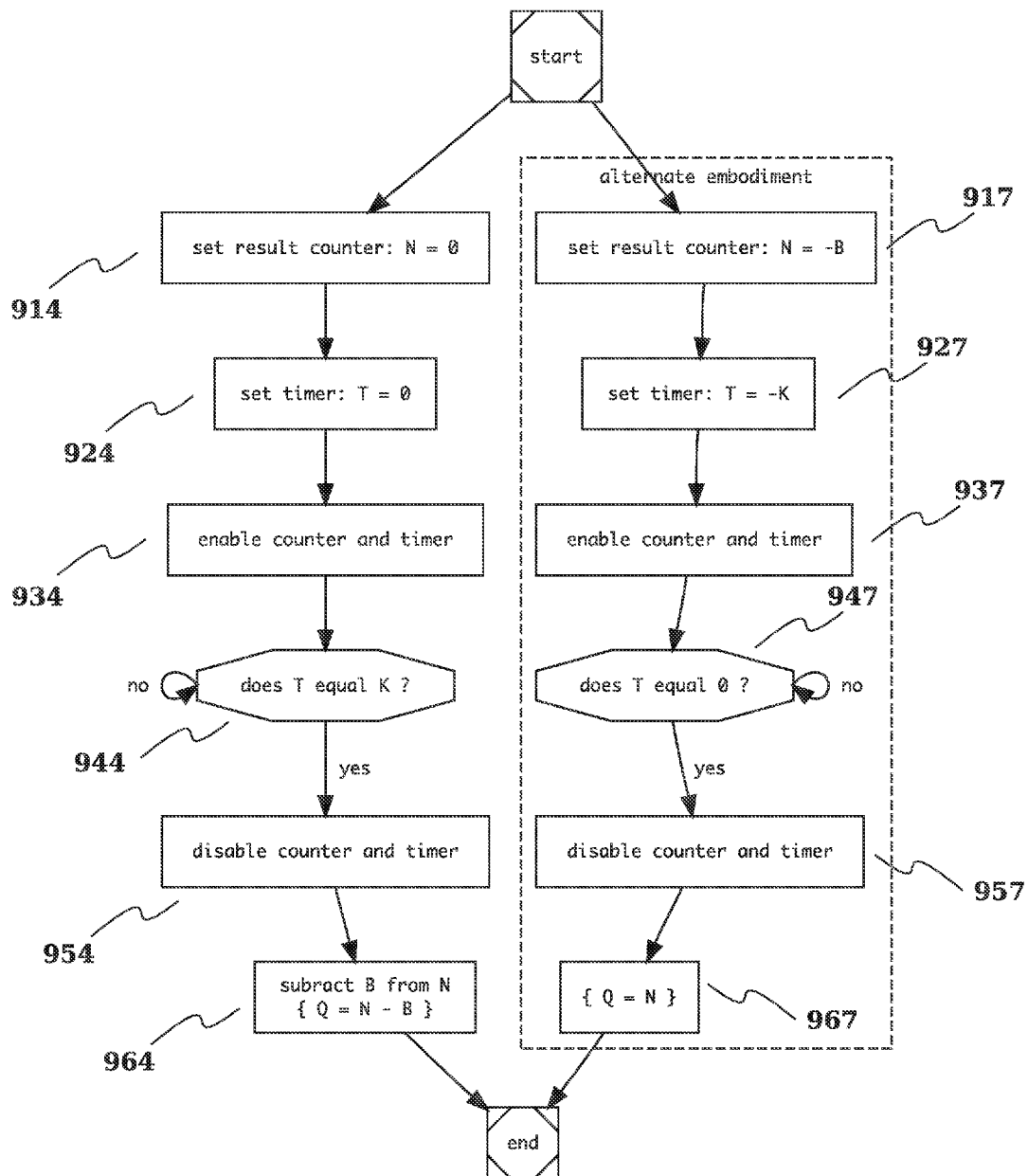
Fig. 13 Count-To-Time Mode
