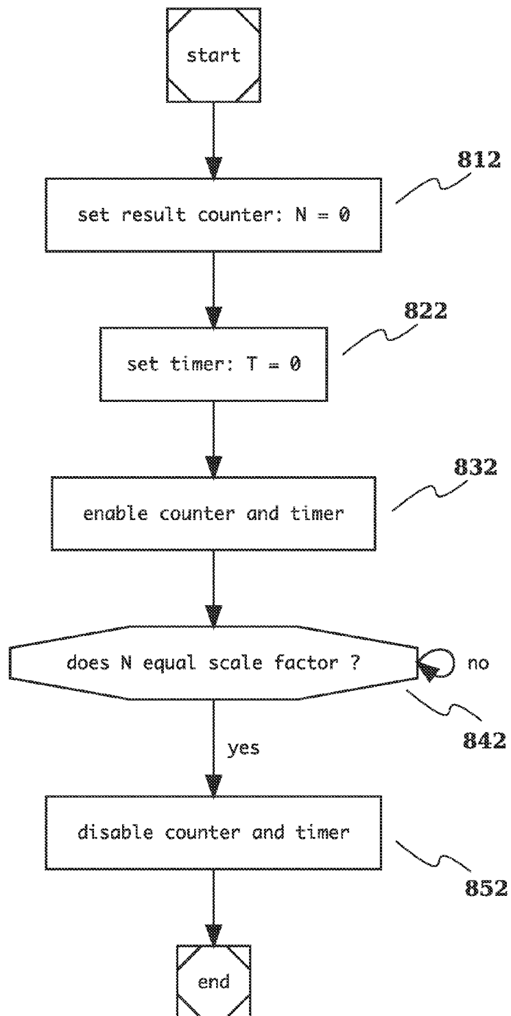
Fig. 10 Calibration Count-To-Time
