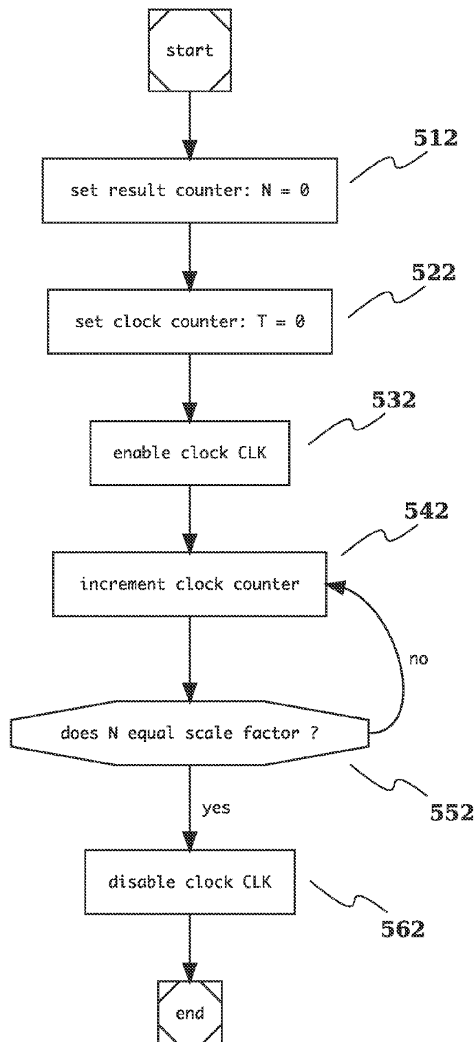
Fig. 6B Calibration Count-To-Time
