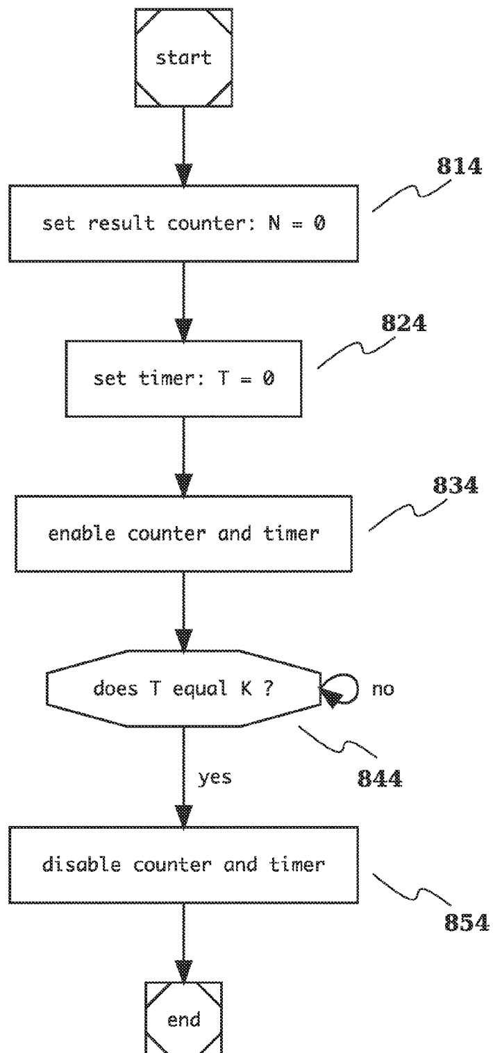
Fig. 11 Calibration Time-To-Count
