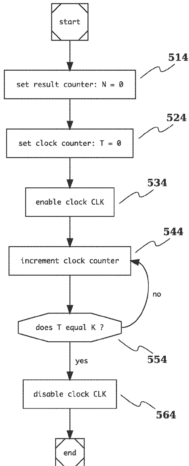
Fig. 6C Calibration Time-To-Count
