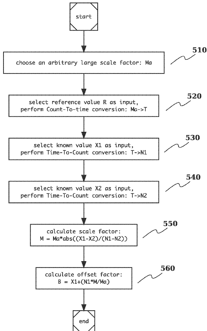
Fig. 6A Dual Mode Converter Calibration
