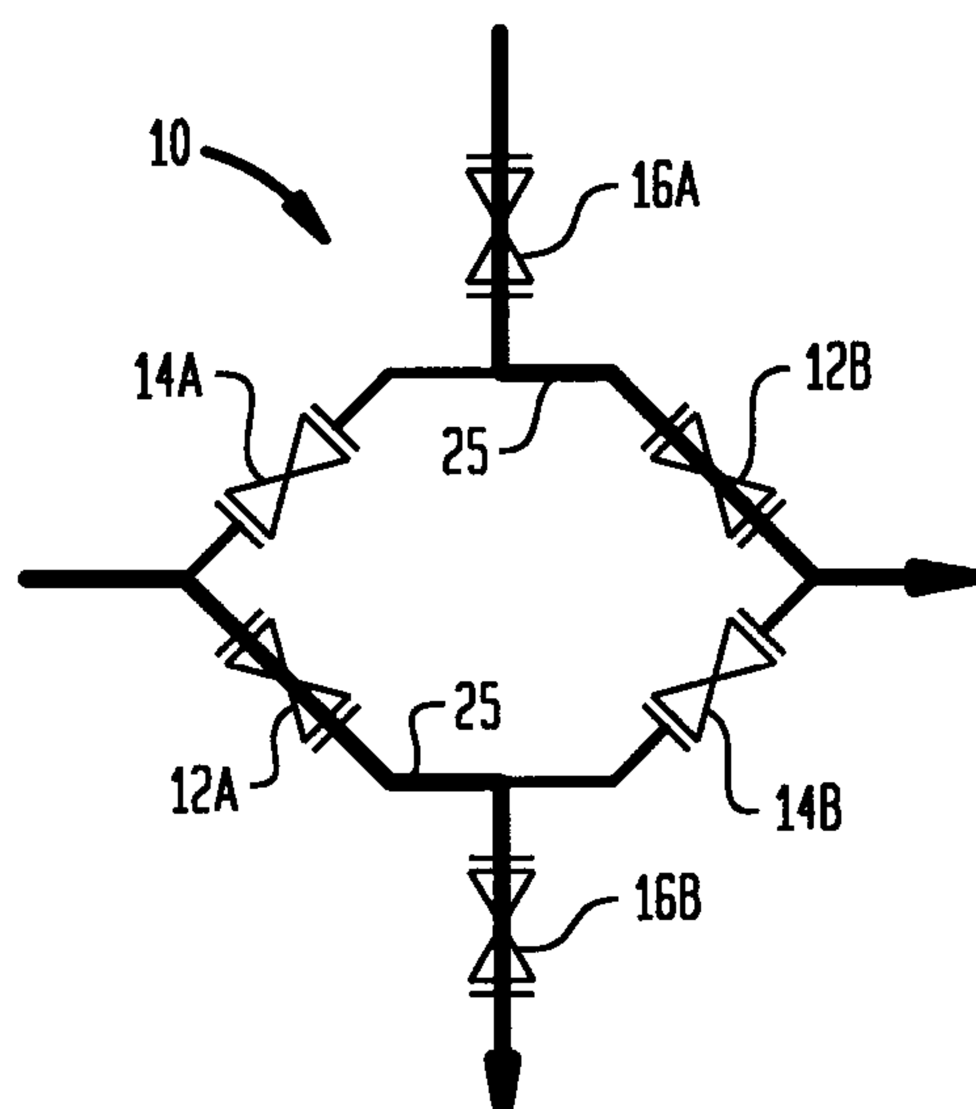
FIG. 1C (PRIOR ART)
