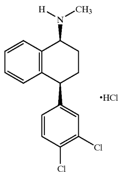
Sertraline hydrochloride
