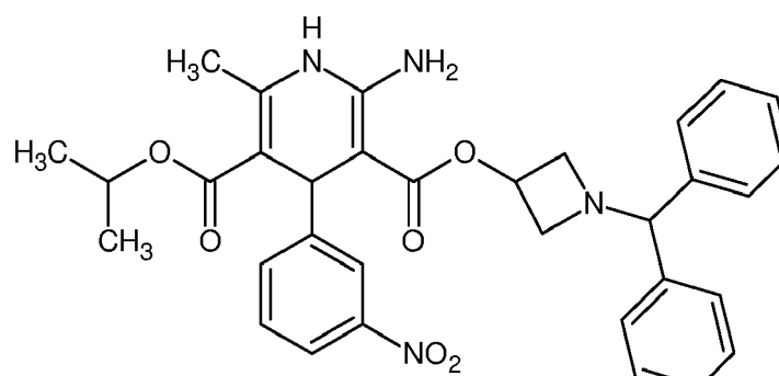
(I-d)
