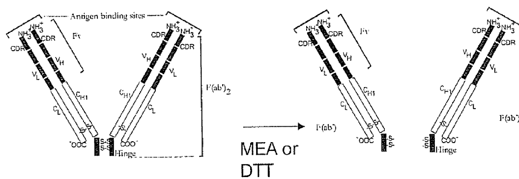
Figure 16: Chemical reduction of a F(ab')_2 fragment to two fully active Fab' fragments.
