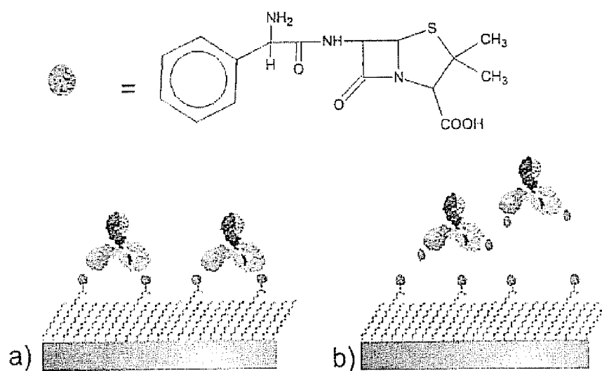
Figure 22 (a) penicillin specific antibodies are bound to the surface modified with the analyte analogue (ampicillin). (b) the surface bound antibodies are replaced by the ampicillin molecules in the sample.
