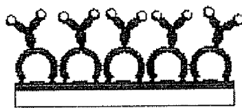
Figure 14: Schematic drawing of an antibody-antigen interaction on a nanoparticle film, covered with self-assembled monolayers of thiols, which bind antibodies, which can bind antigen.
