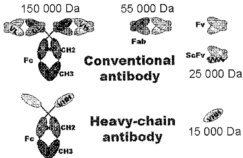
Figure 17 Top: Conventional antibody structure and its fragments (Fab, Fv, ScFv). Bottom: Heavy Chain antibody and its VHH fragment
