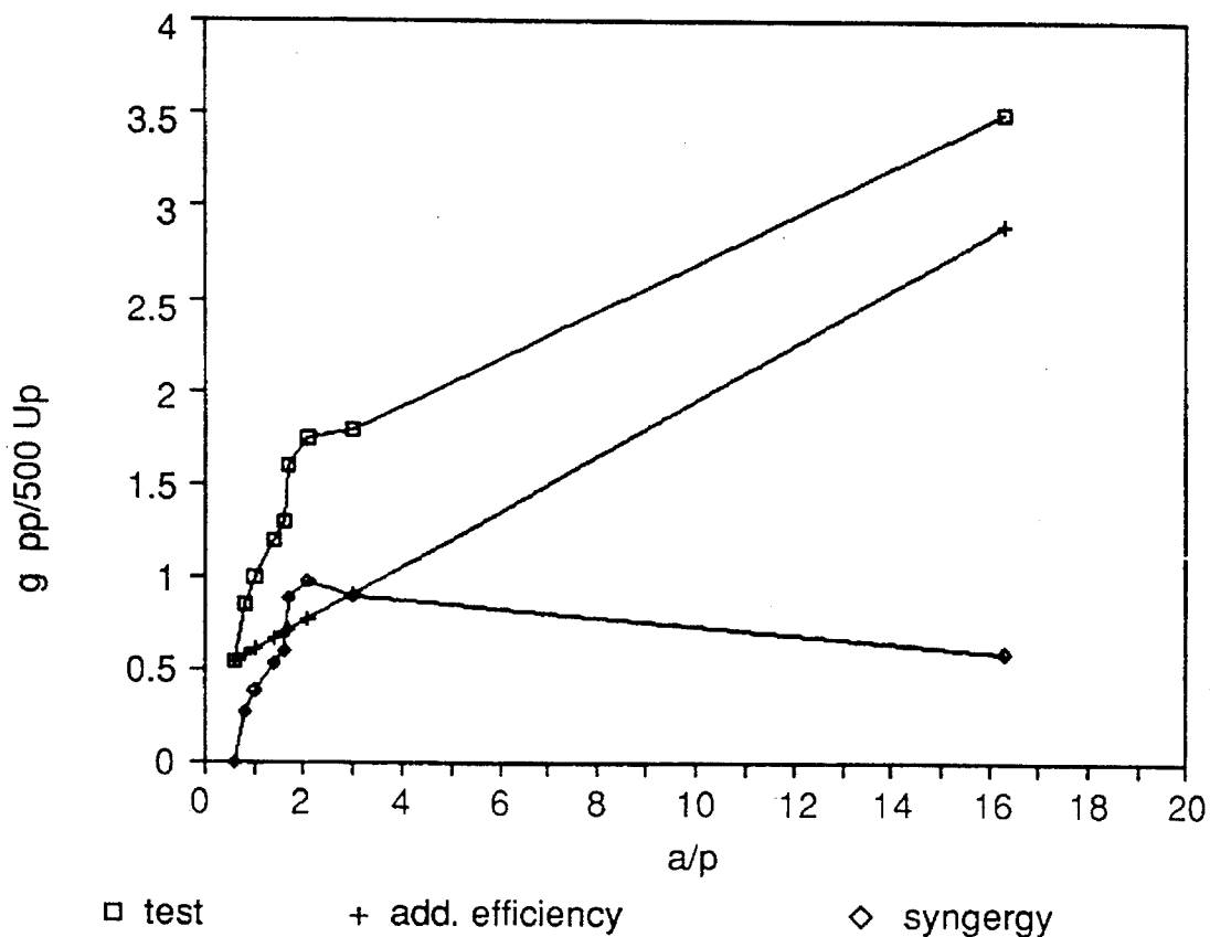
in vitro synergetic effect between phytase 0.6/1 and acid phosphatase 1/0 in different A. ficuum phytase preparations.
