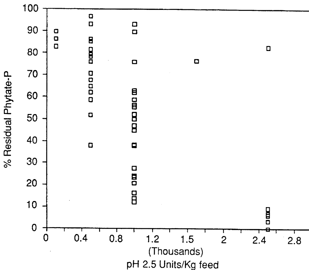
in vitro phytin hydrolysis by A. ficuum phytase preparations in function of pH 2.5 activity
