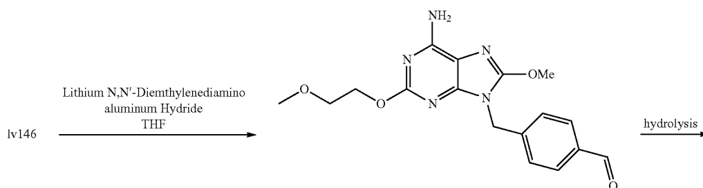
148 4-[6-Amino-8-methoxy-2-(2-methoxyethoxy)-purin-9-ylmethyl]-benzaldehyde
