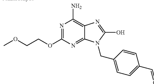
150 4-[6-Amino-8-methoxy-2-(2-hydroxyethoxy)-purin-9-ylmethyl]-benzaldehyde
