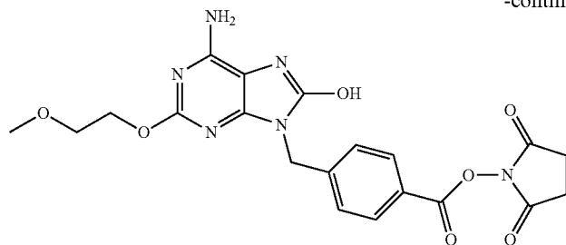
2,5-dioxypyrrolidin-1-yl 4-((6-amino-8-hydroxy-2-(2-methoxyethoxy)-9H-purin-9-yl)methyl)benzoate
