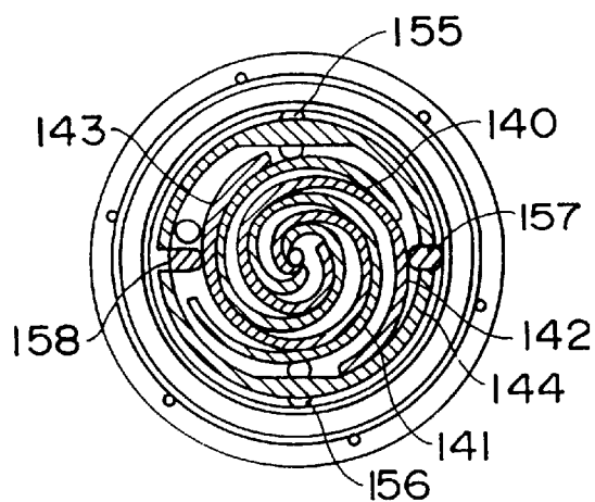
FIG. 10 (PRIOR ART)
