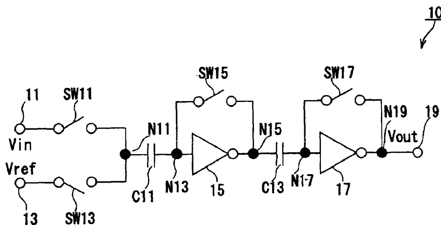
FIG. 2-1 (PRIOR ART)
