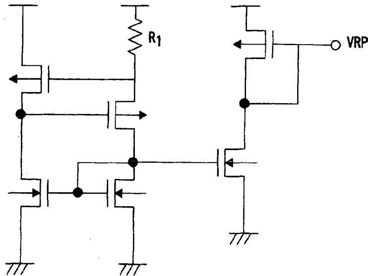
CIRCUIT DIAGRAM SHOWING A CONFIGURATION OF A REFERENCE VOLTAGE CIRCUIT
