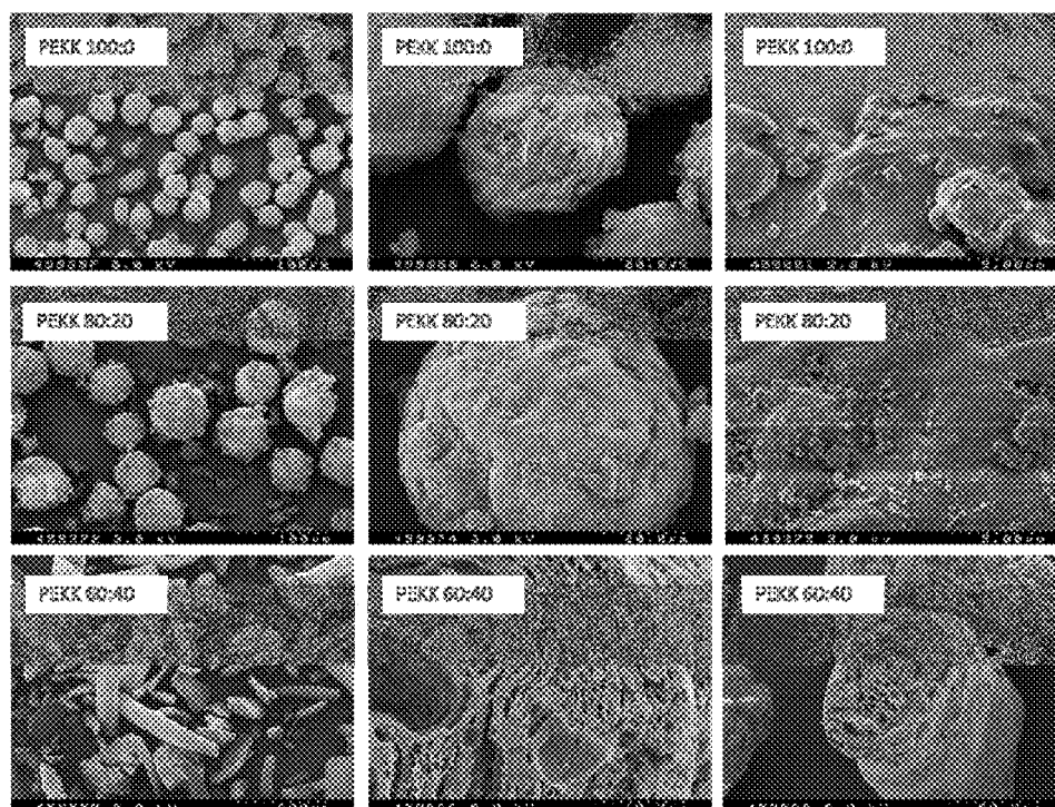
FIG. 1 Reactive end cap PEKK polymer particles with different T:I ratios
