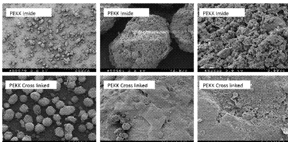
FIG. 2 Copolymer backbone PEKK imide and cross-linked versions at different magnifications showing size, shape, and surface feature
