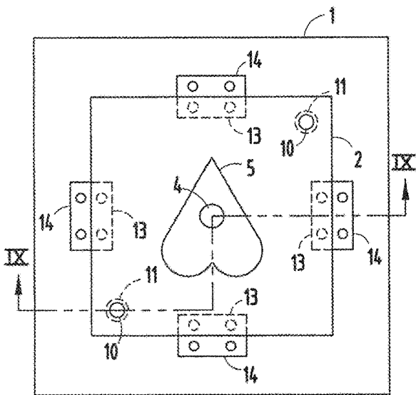
FIG. 8 PRIOR ART
