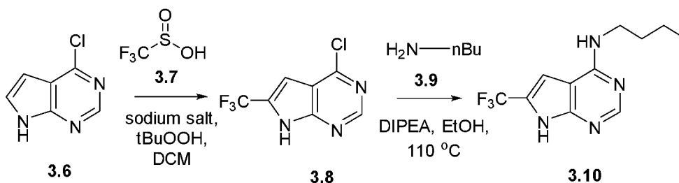
SCHEME 3B.
