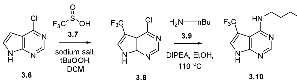
SCHEME 3B.
