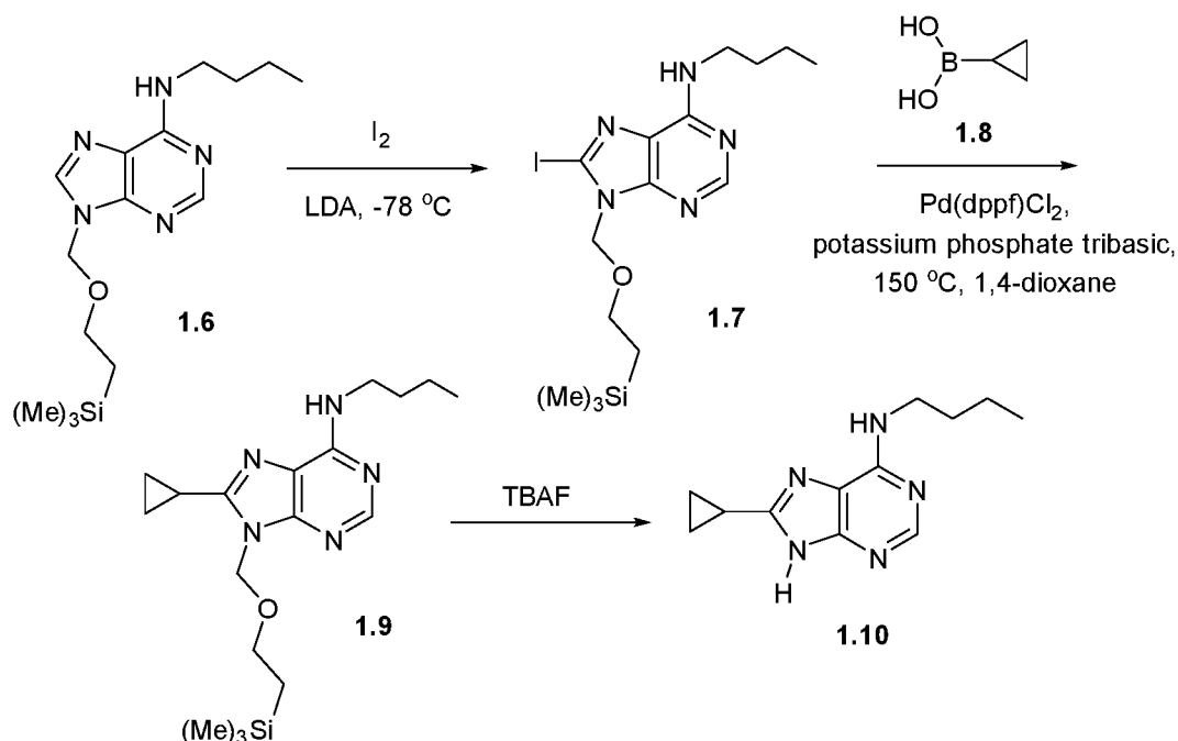
SCHEME 1B.
