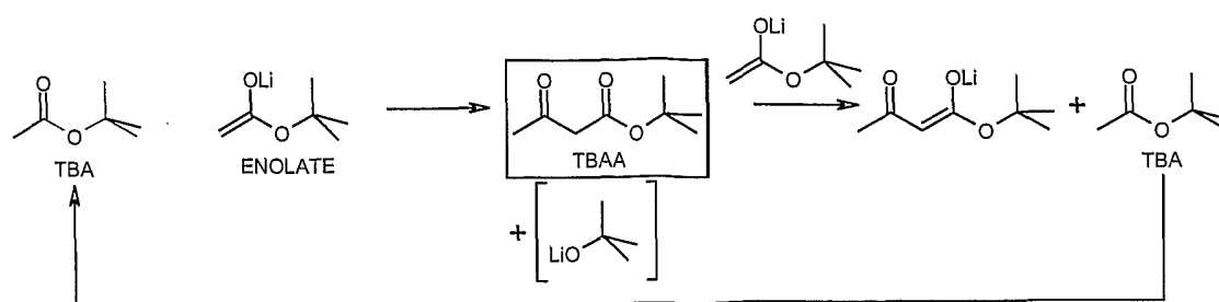
Scheme 1 : Self condensation of alkyl acetate enolate
