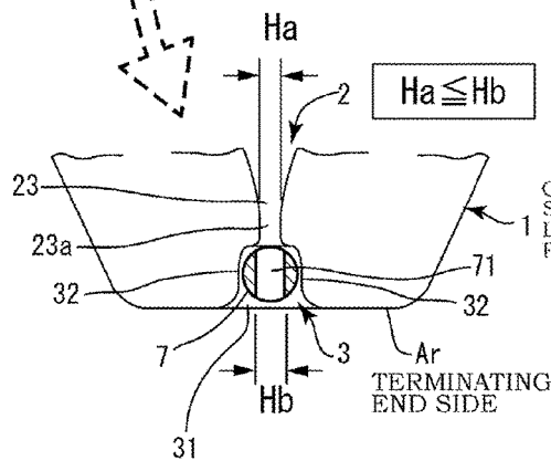
ENLARGED VIEW OF (α)-PART
