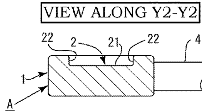
VIEW ALONG Y2-Y2
