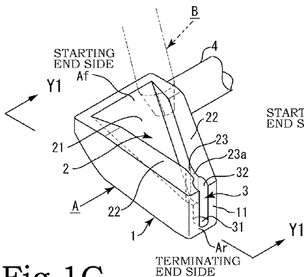
VIEW ALONG Y1-Y1
