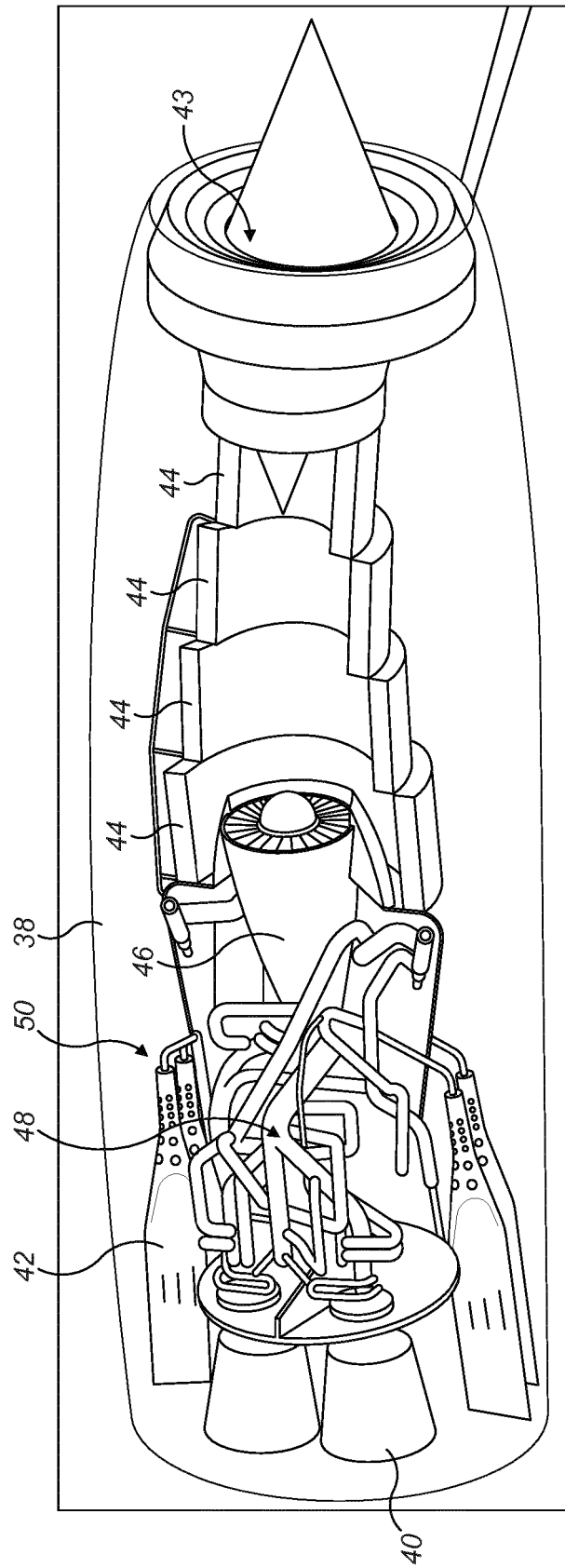
FIG. 2 Prior Art
