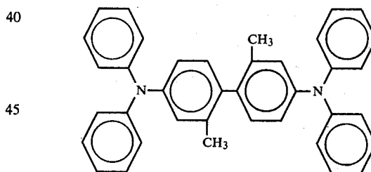
N,N,N',N'-Tetra-(4-methylphenyl)-[2,2'-dimethyl-1,1'-biphenyl]-4,4'-diamine;
