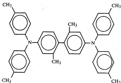
N,N,N',N'-Tetra(4-methylphenyl)-[2,2'-dimethyl-1,1'-biphenyl]-4,4'-diamine:
