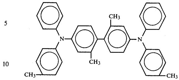
N,N'-Diphenyl-N,N'-bis(4-methylphenyl)-[2,2'-dimethyl-1,1'-biphenyl]-4,4'-diamine.
