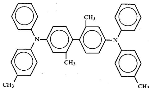
N,N'-Diphenyl-N,N'-bis(4-methylphenyl)-[2,2'-dimethyl-1,1'-biphenyl]-4,4'-diamine;
