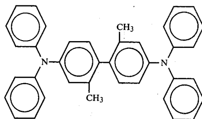
N,N,N',N'-Tetra(4-methylphenyl)-[2,2'-dimethyl-1,1'-biphenyl]-4,4'-diamine:
