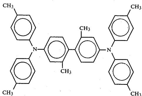
N,N'-Diphenyl-N,N'-bis(4-methylphenyl)-[2,2'-dimethyl-1,1'-biphenyl]-4,4'-diamine;
