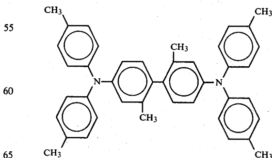
N,N'-Diphenyl-N,N'-bis(4-methylphenyl)-[2,2'-dimethyl-1,1'-biphenyl]-4,4'-diamine;
