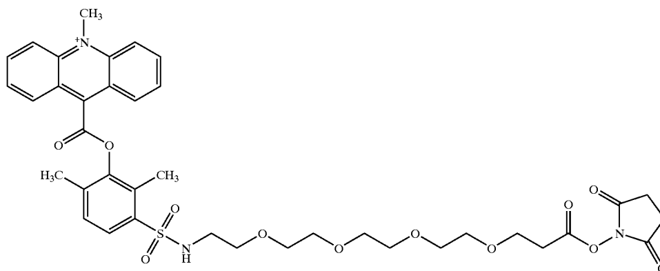
MeAE-PEO4-NHS
