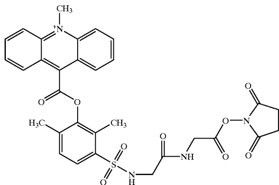
MeAE-Gly2-NHS
