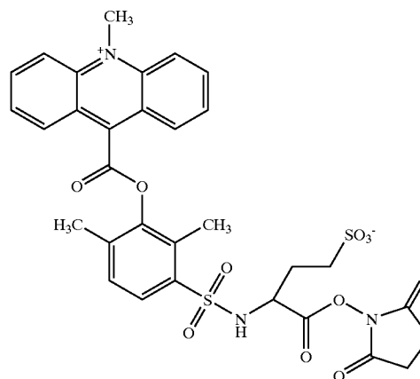
MeAE-HCA-NHS
