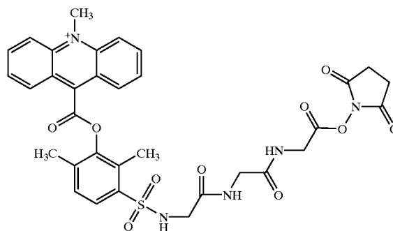
MeAE-Gly3-NHS
