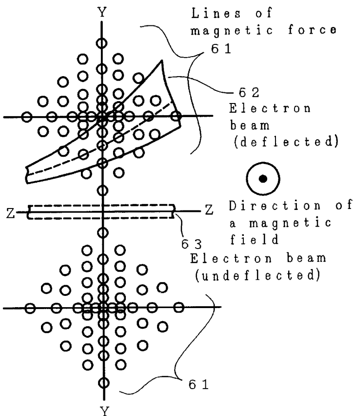
Direction of an electron beam travel
