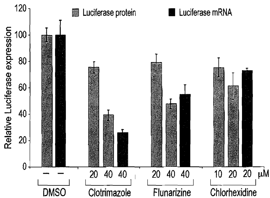
Clotrimazole
