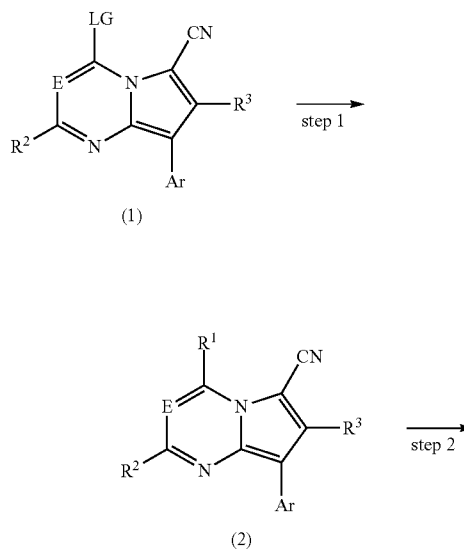
Reaction Scheme 1
