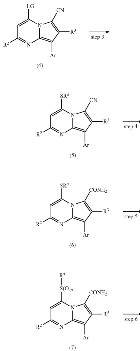
Reaction Scheme 2
