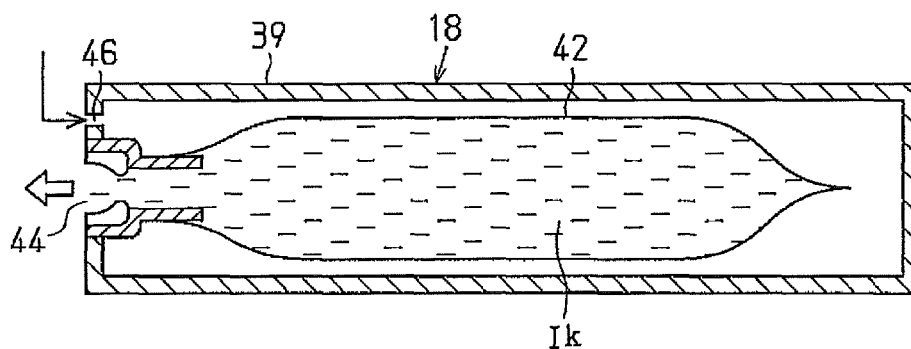
Fig. 25 (Prior Art)
