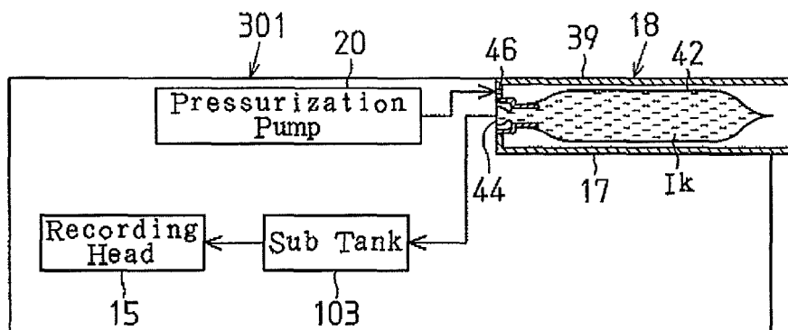
Fig. 24 (Prior Art)
