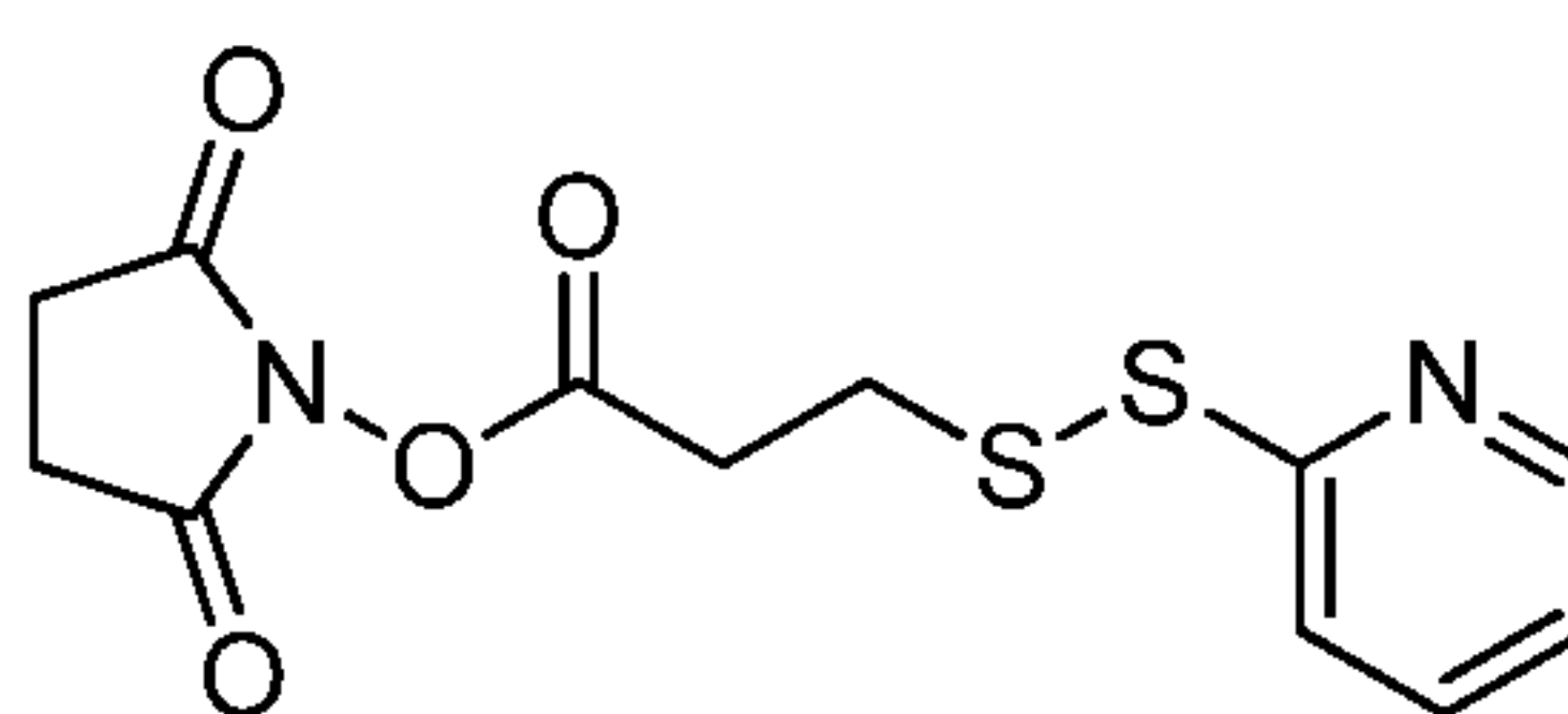
N -succinimidyl-3-(2-pyridyldithio)propionate (SPDP),
