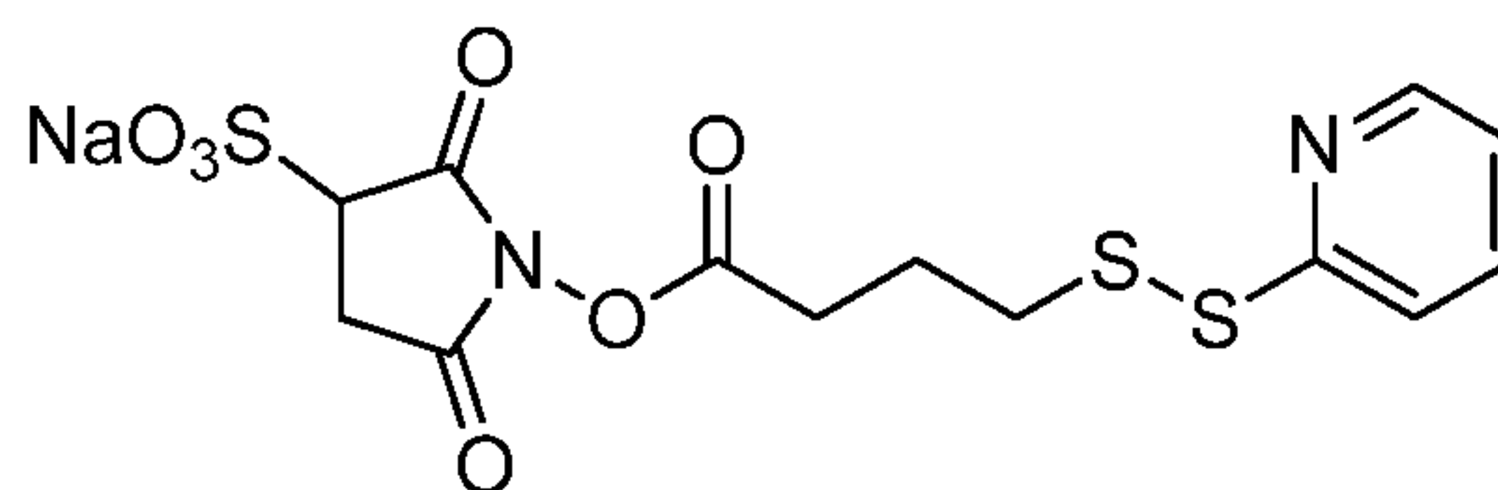
N-succinimidyl-4-(2-pyridyldithio)2-sulfo-butanoate (sulfo-SPDB).
