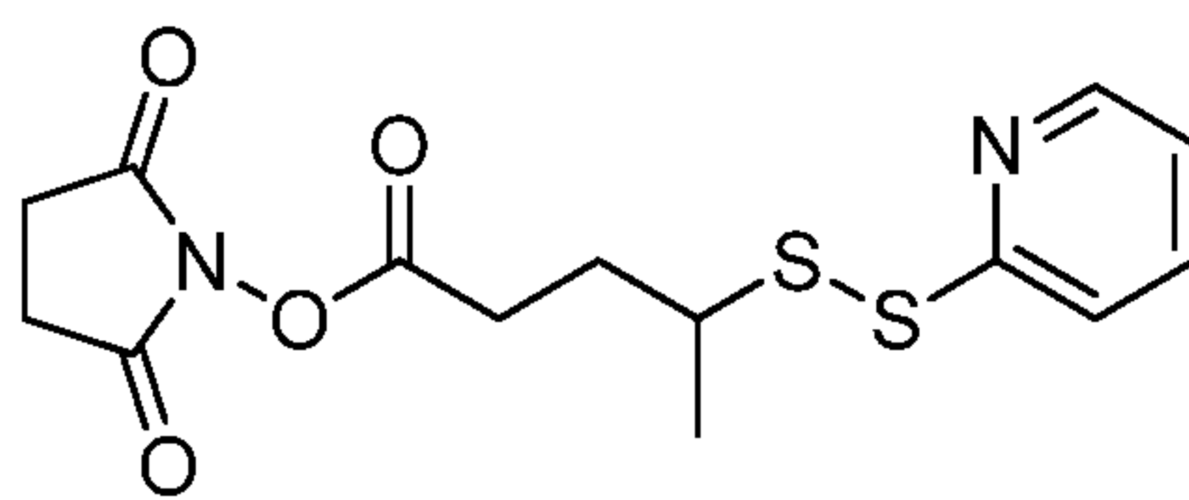
N-succinimidyl-4-(2-pyridyldithio)pentanoate (SPP),
