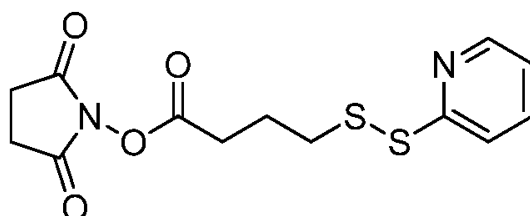
N-succinimidyl-4-(2-pyridyldithio)butanoate (SPDB) and
