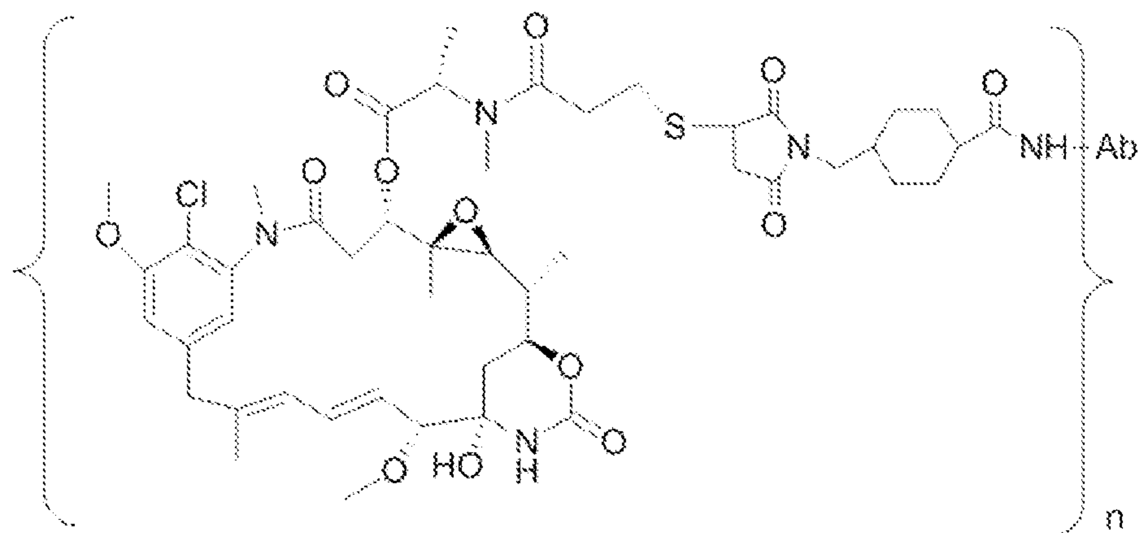
Ab-MCC-DM1
