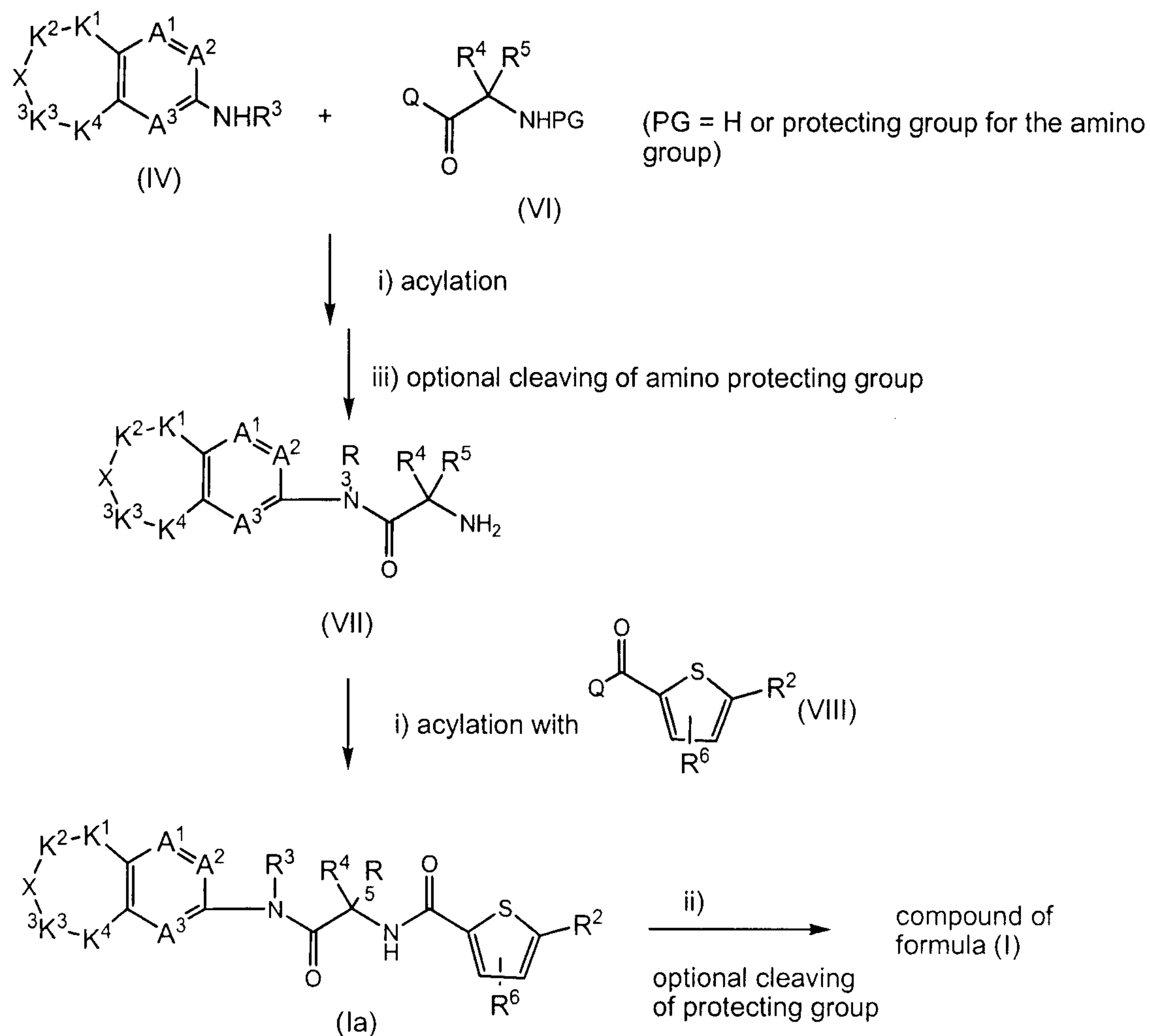
Scheme 2
