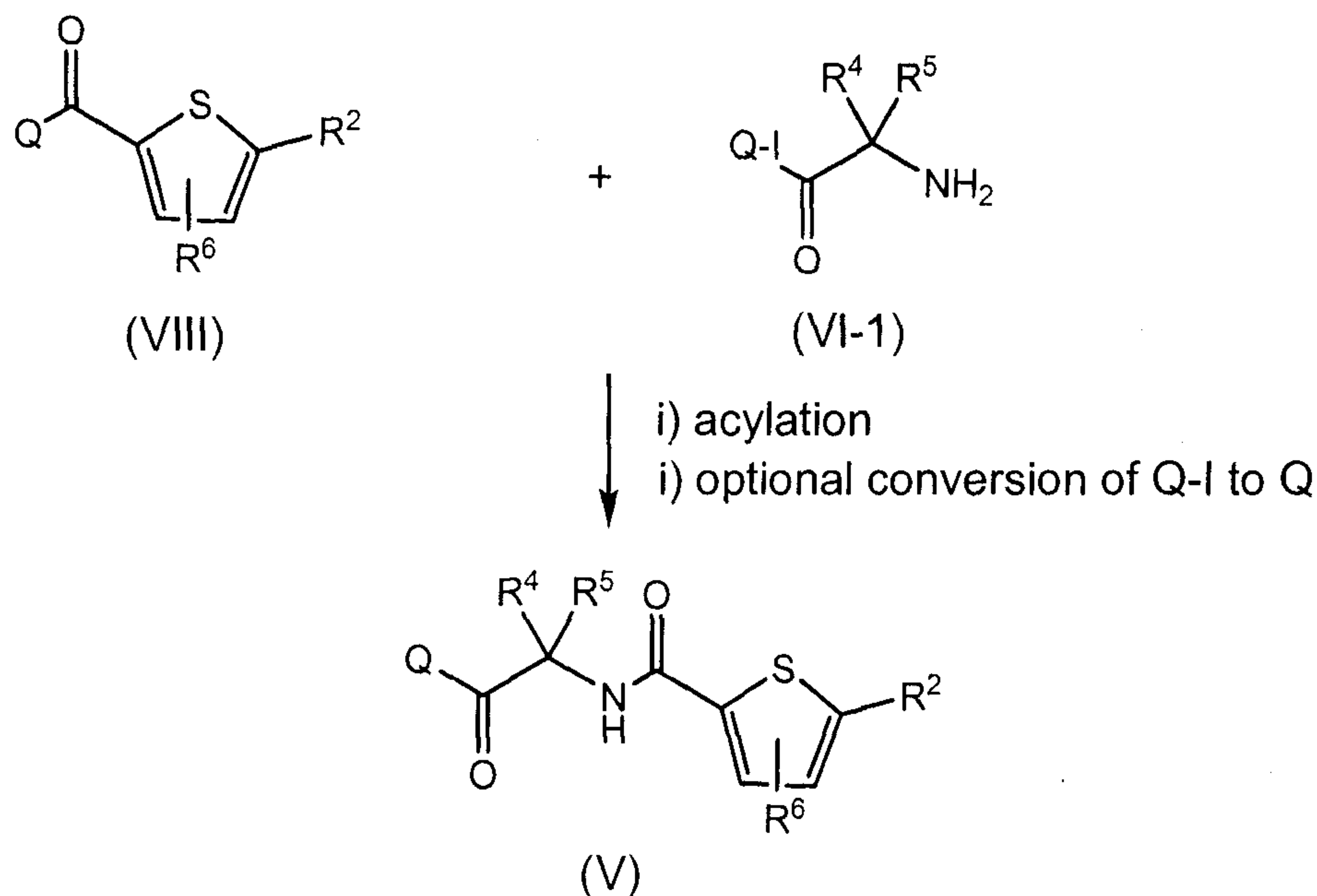
Scheme 3
