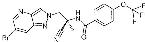
Compound 3.024
