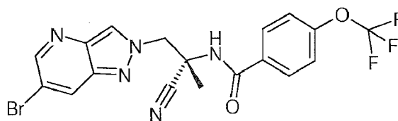
Compound 3.025
