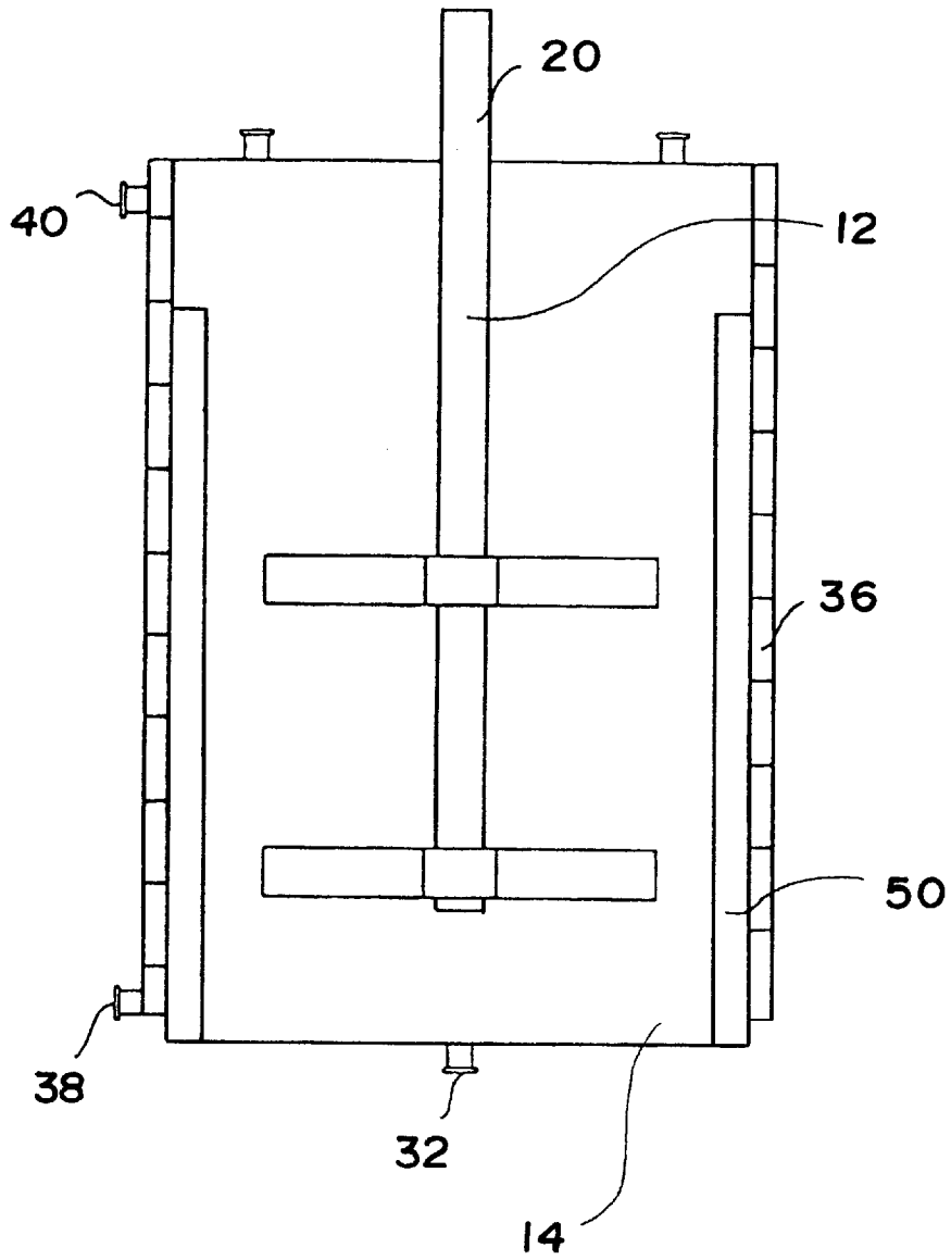
FIG. 5 PRIOR ART
