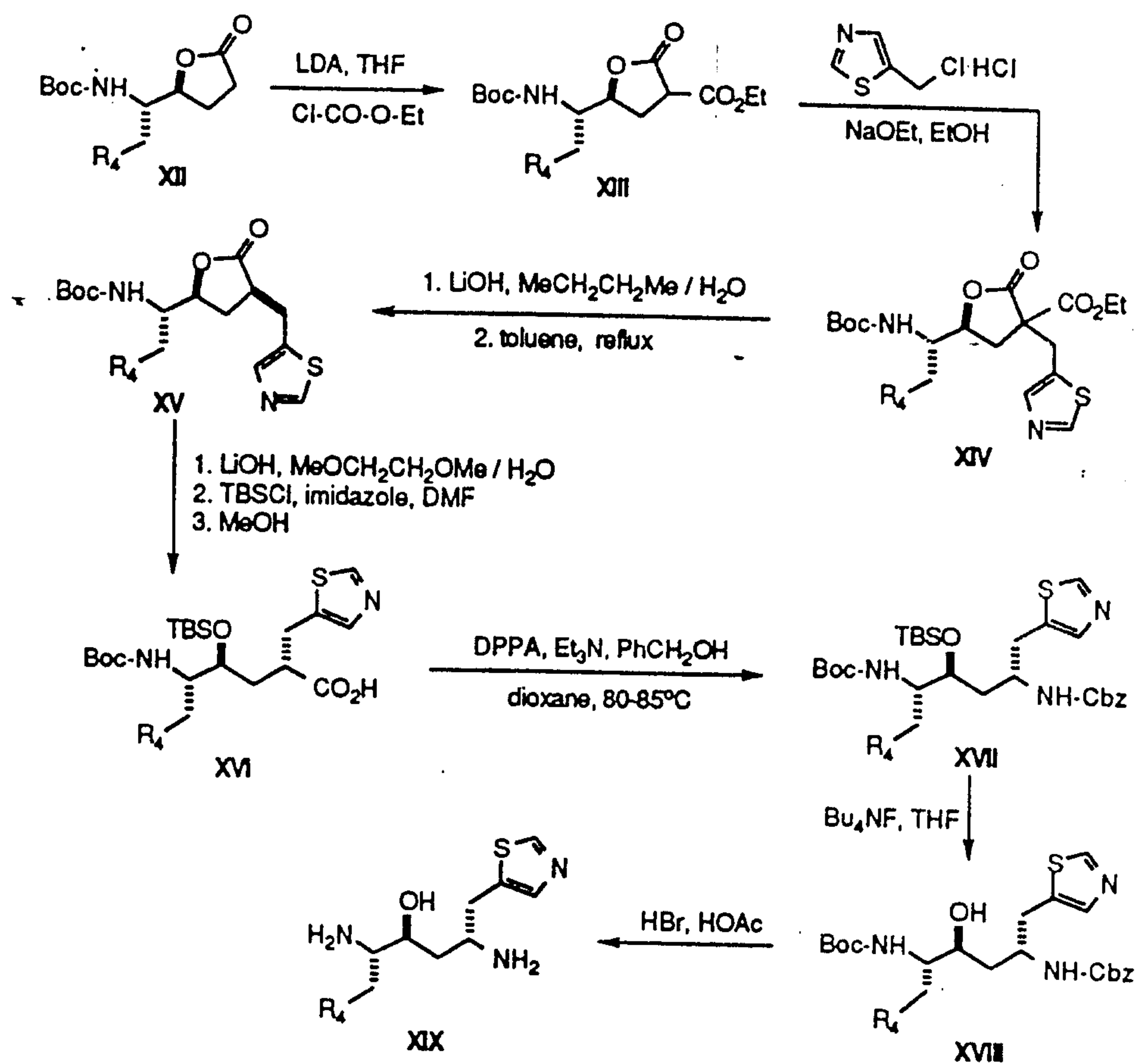
Scheme 3
