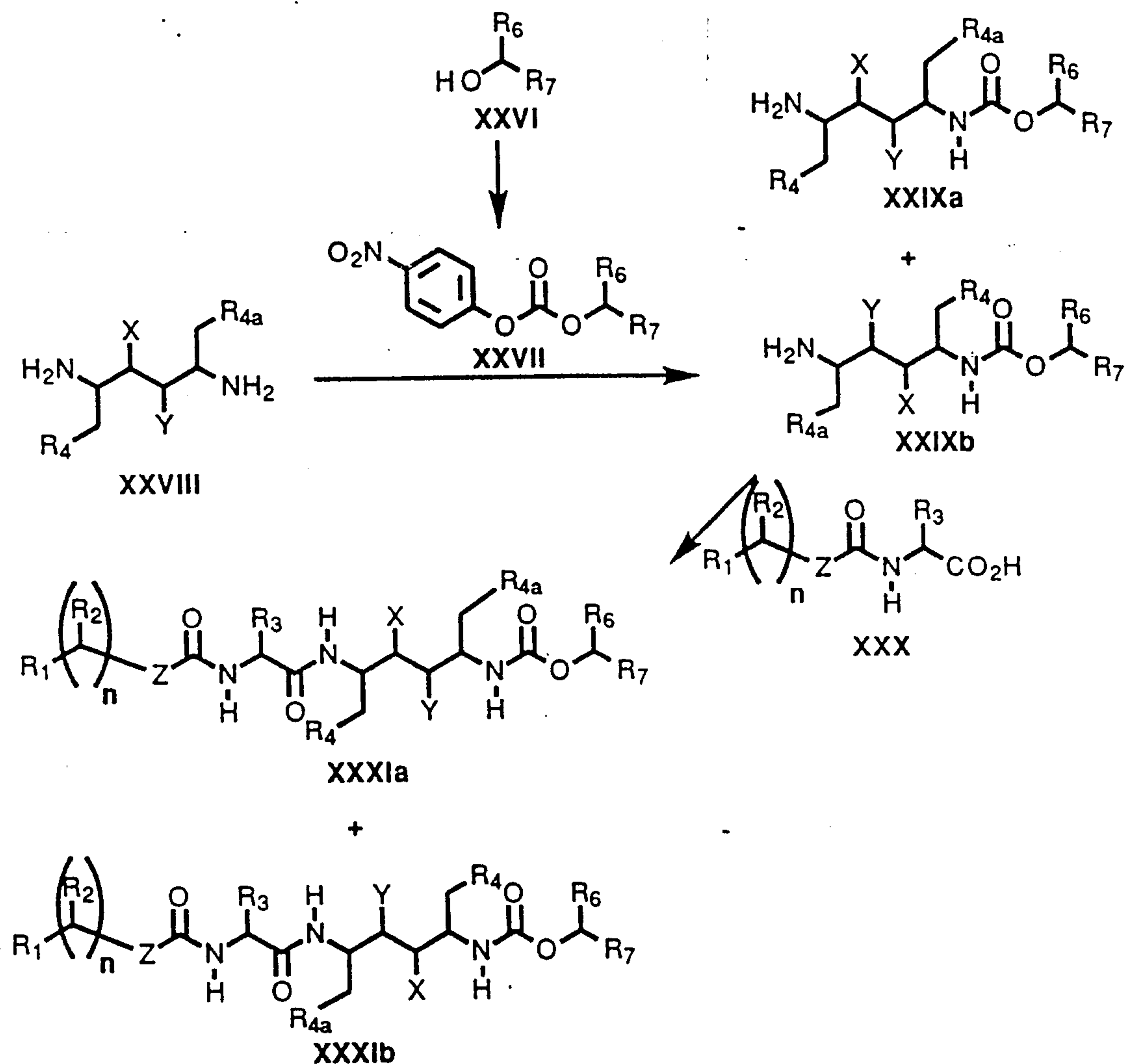
Scheme 5
