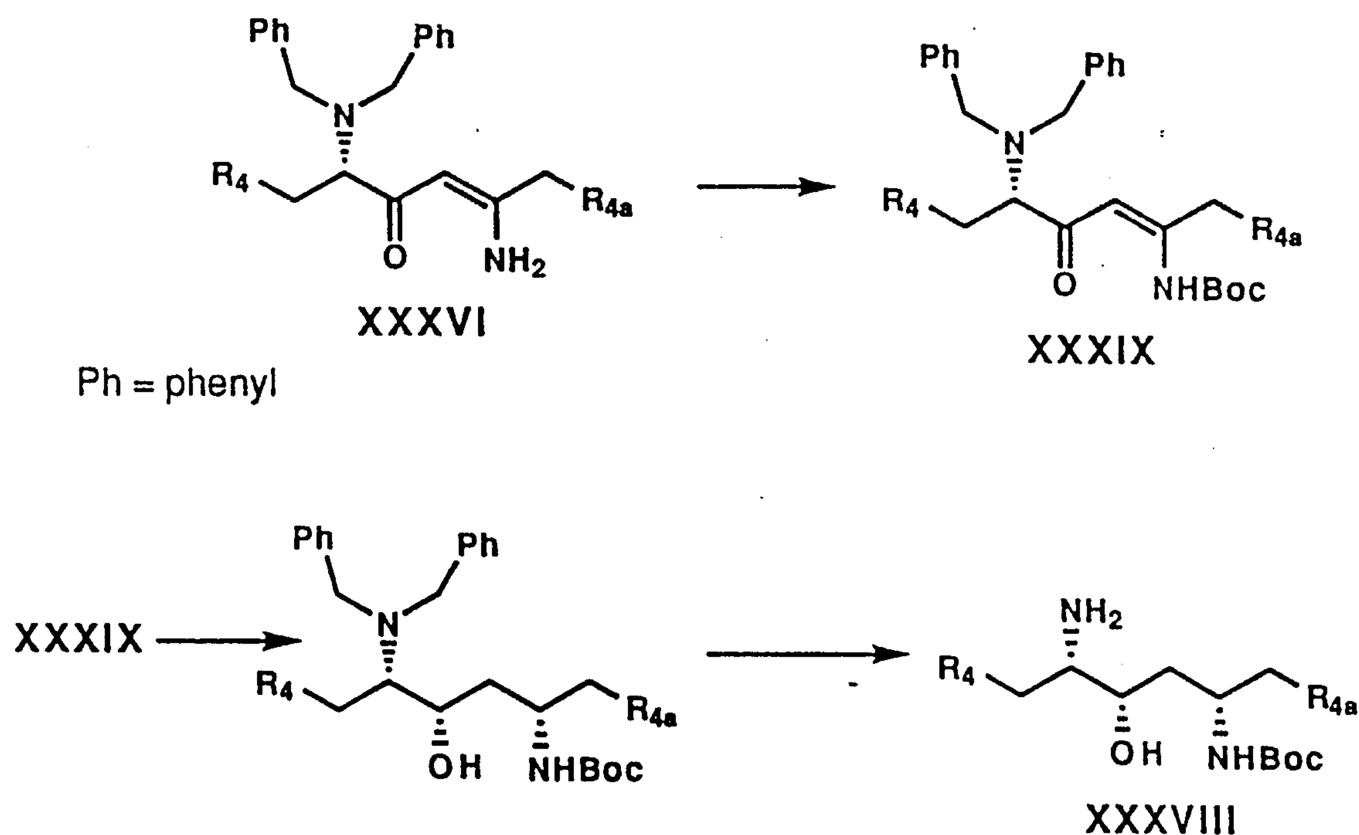
Scheme 8
