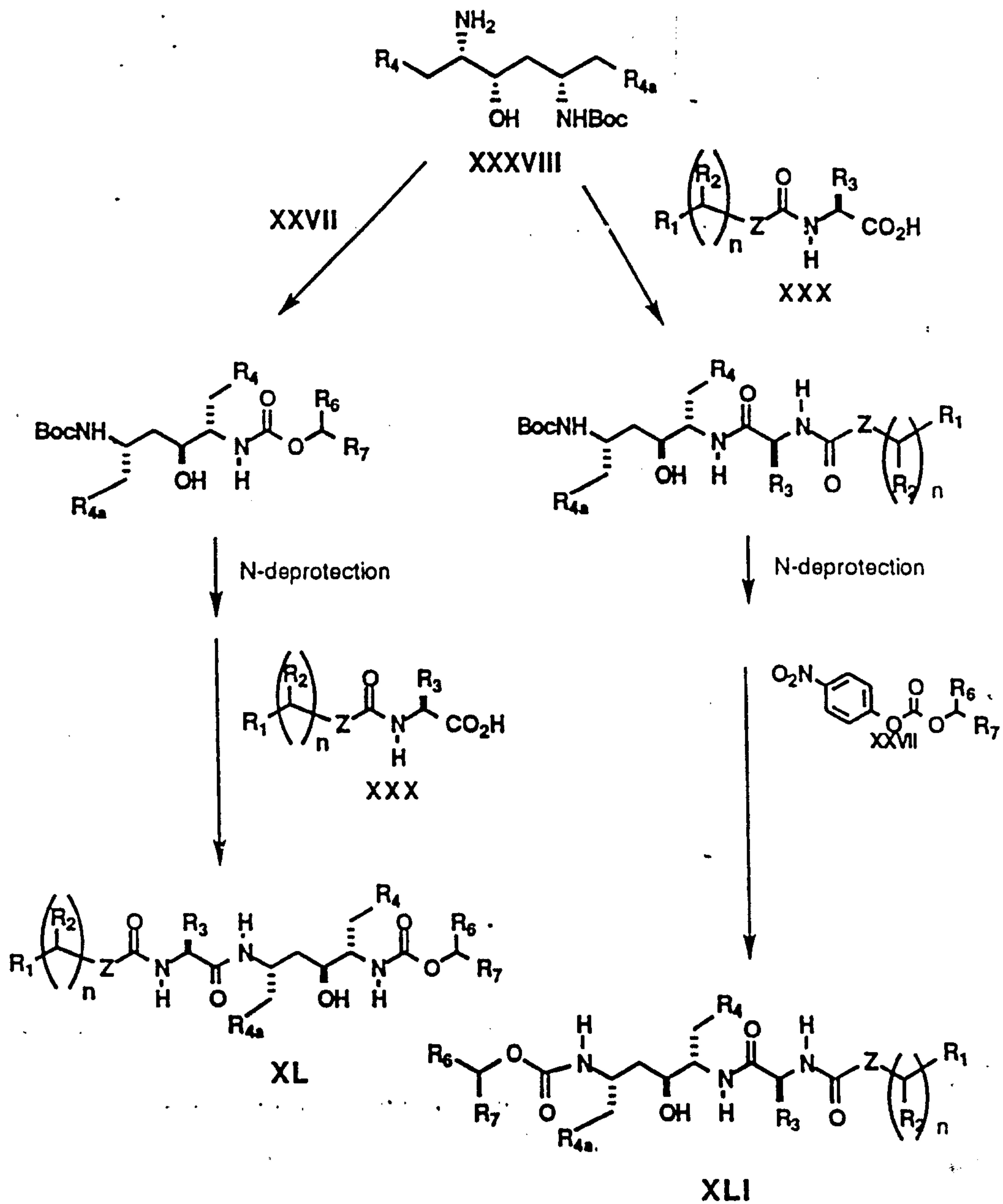
Scheme 9
