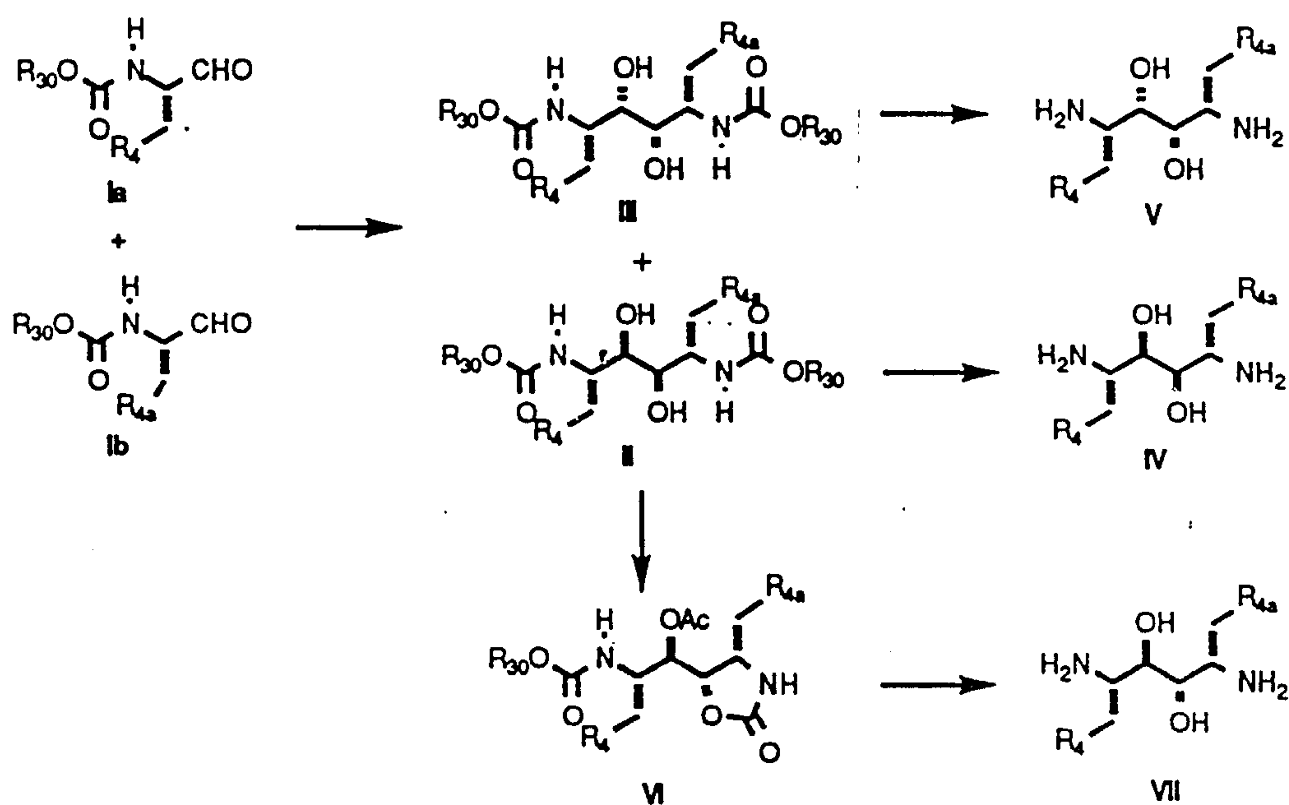
Scheme 1
