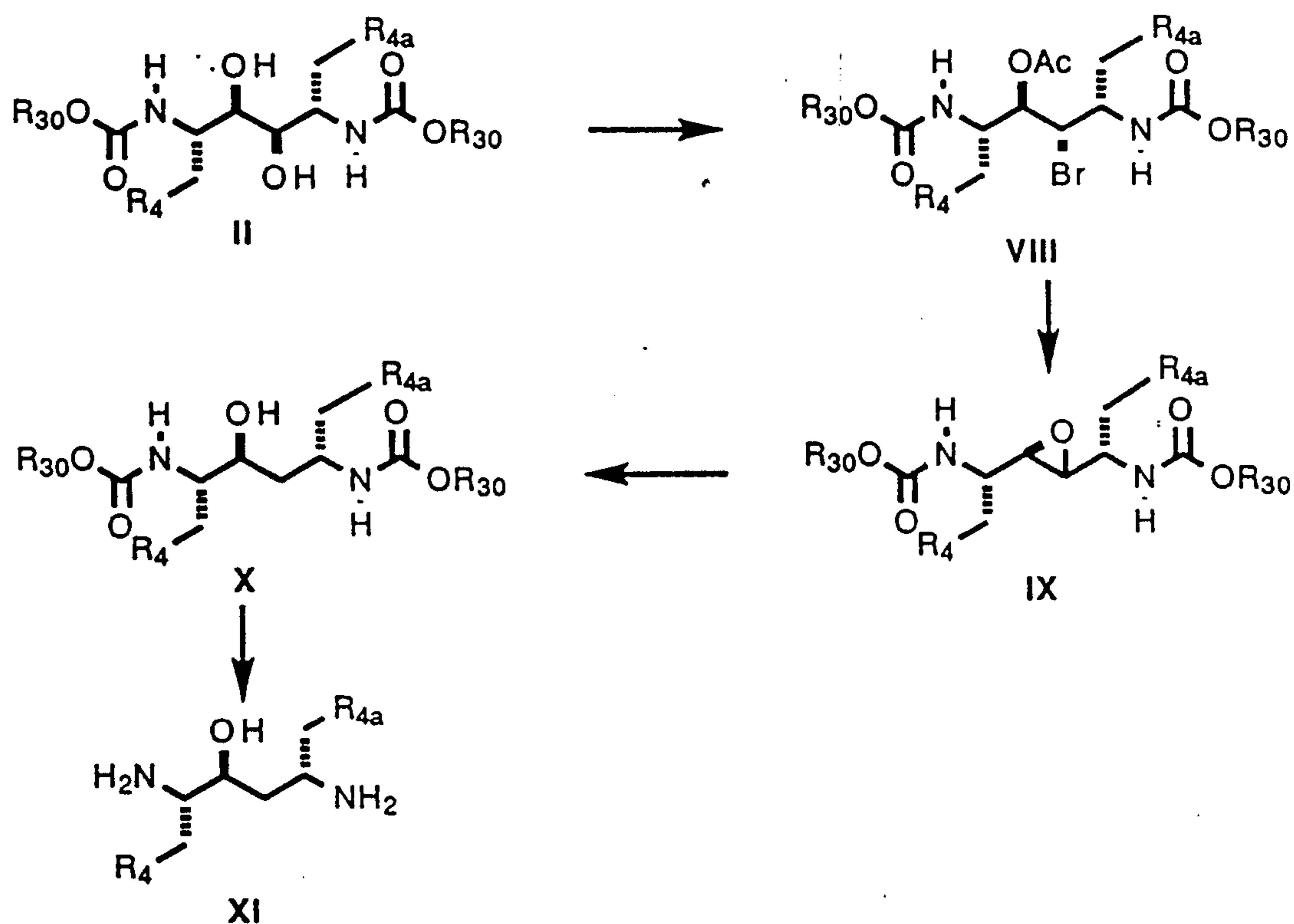
Scheme 2
