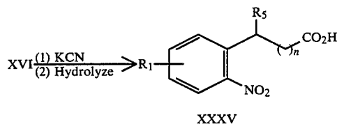
Equation 24
