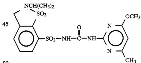
Compound 9
