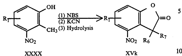
Equation 34
