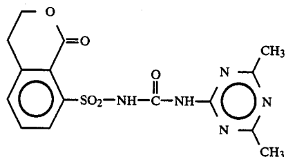
Compound 72
