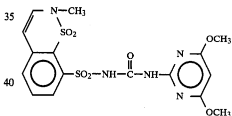
Compound 71
