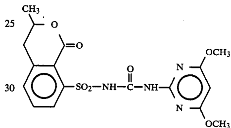
Compound 76
