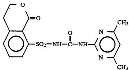
Compound 70
