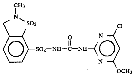
Compound 6
