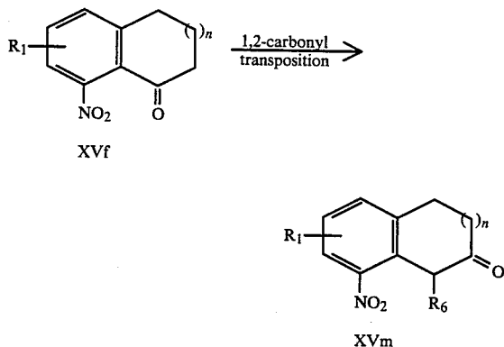
Equation 39
