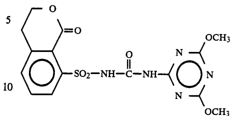
Compound 69
