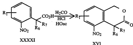
Equation 35
