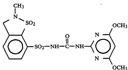
Compound 5
