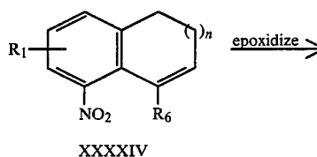
Equation 37
