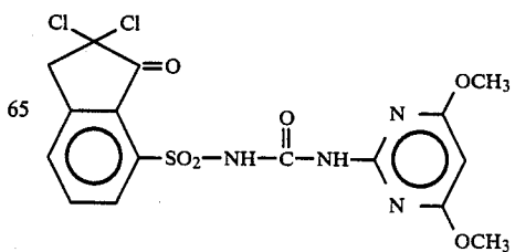
Compound 80
