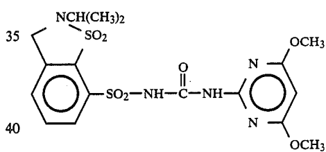
Compound 8
