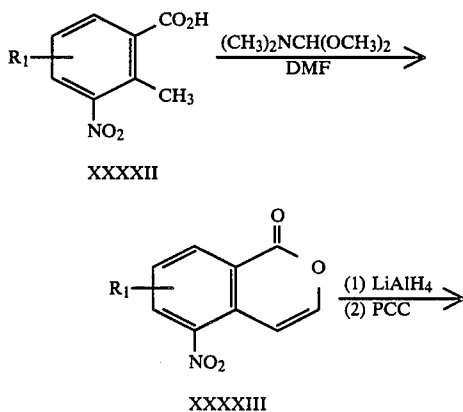
Equation 36
