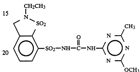
Compound 6
