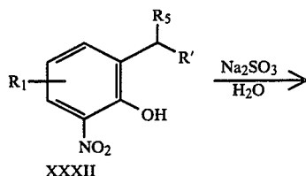
Equation 27
