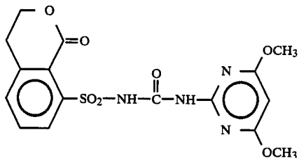
Compound 71
