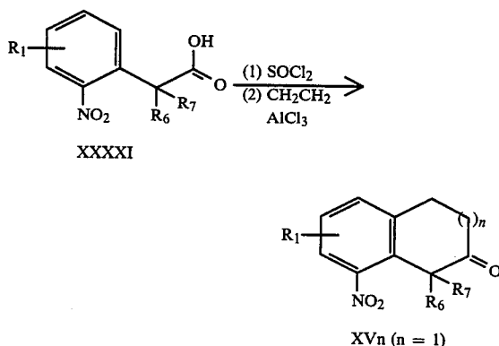
Equation 38
