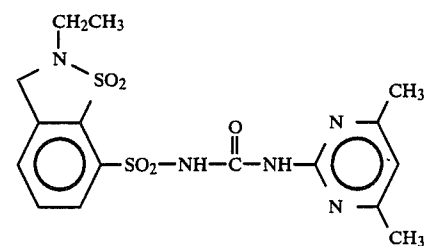
Compound 9
