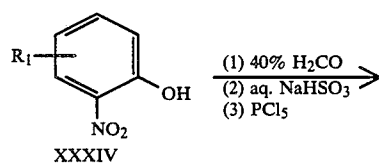
Equation 28
