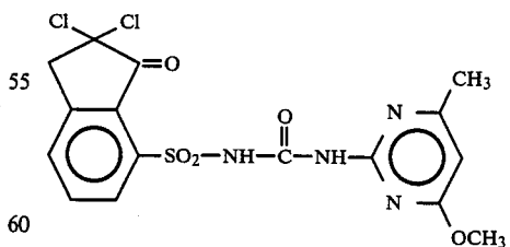
Compound 73
