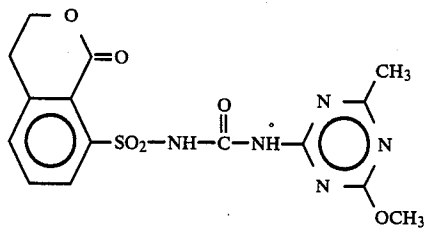
Compound 73
