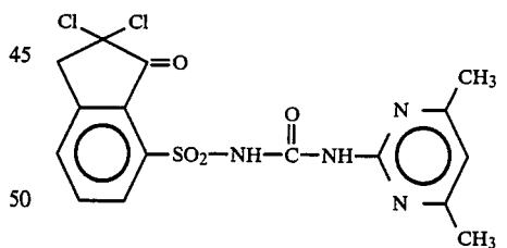
Compound 72
