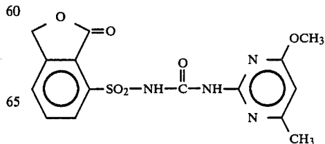
Compound 17
