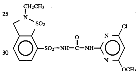
Compound 7
