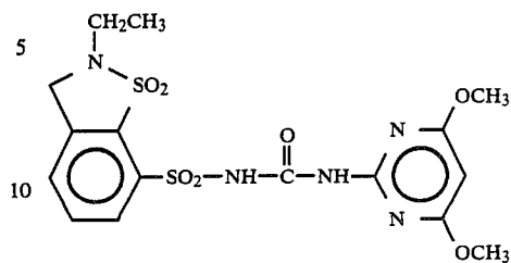
Compound 11
