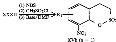
Equation 29
