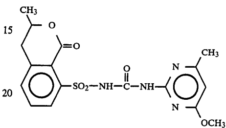
Compound 70
