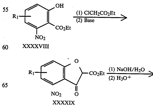
Equation 41
