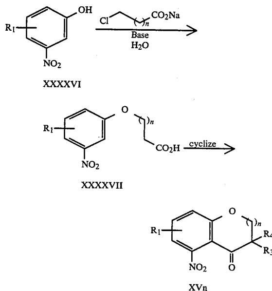
Equation 40
