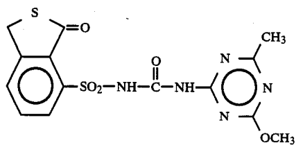
Compound 69
