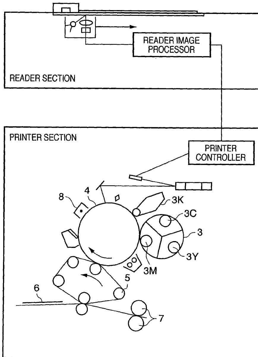
FIG. 24 Prior Art
