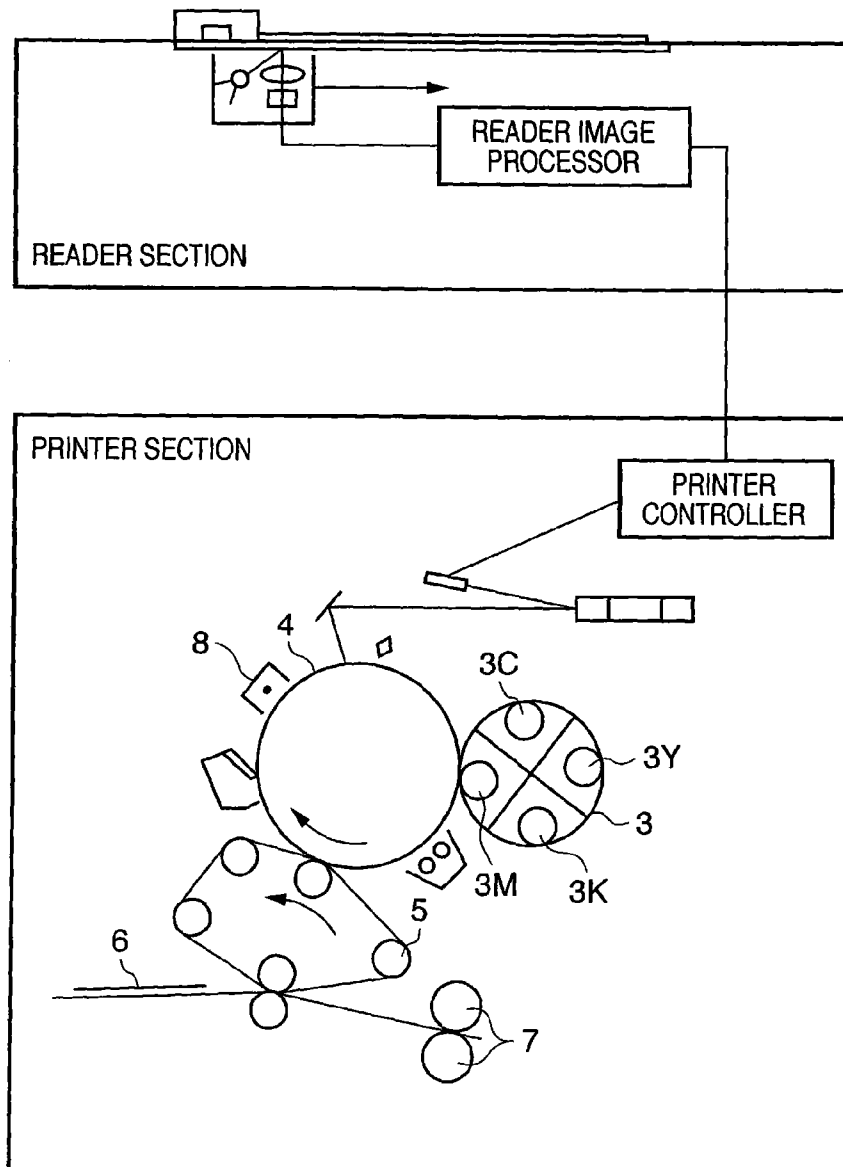
FIG. 23 Prior Art
