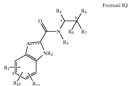
Formula IQ
