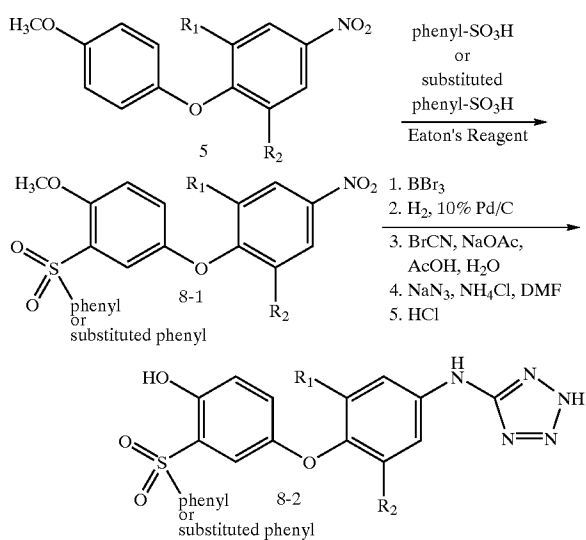
Scheme 8
