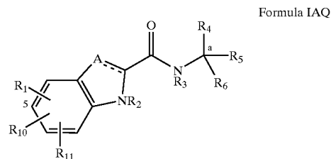
Formula IAQ
