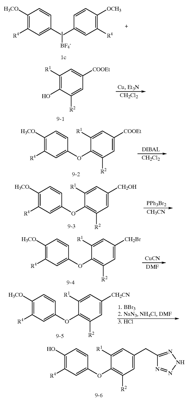
Scheme 9
