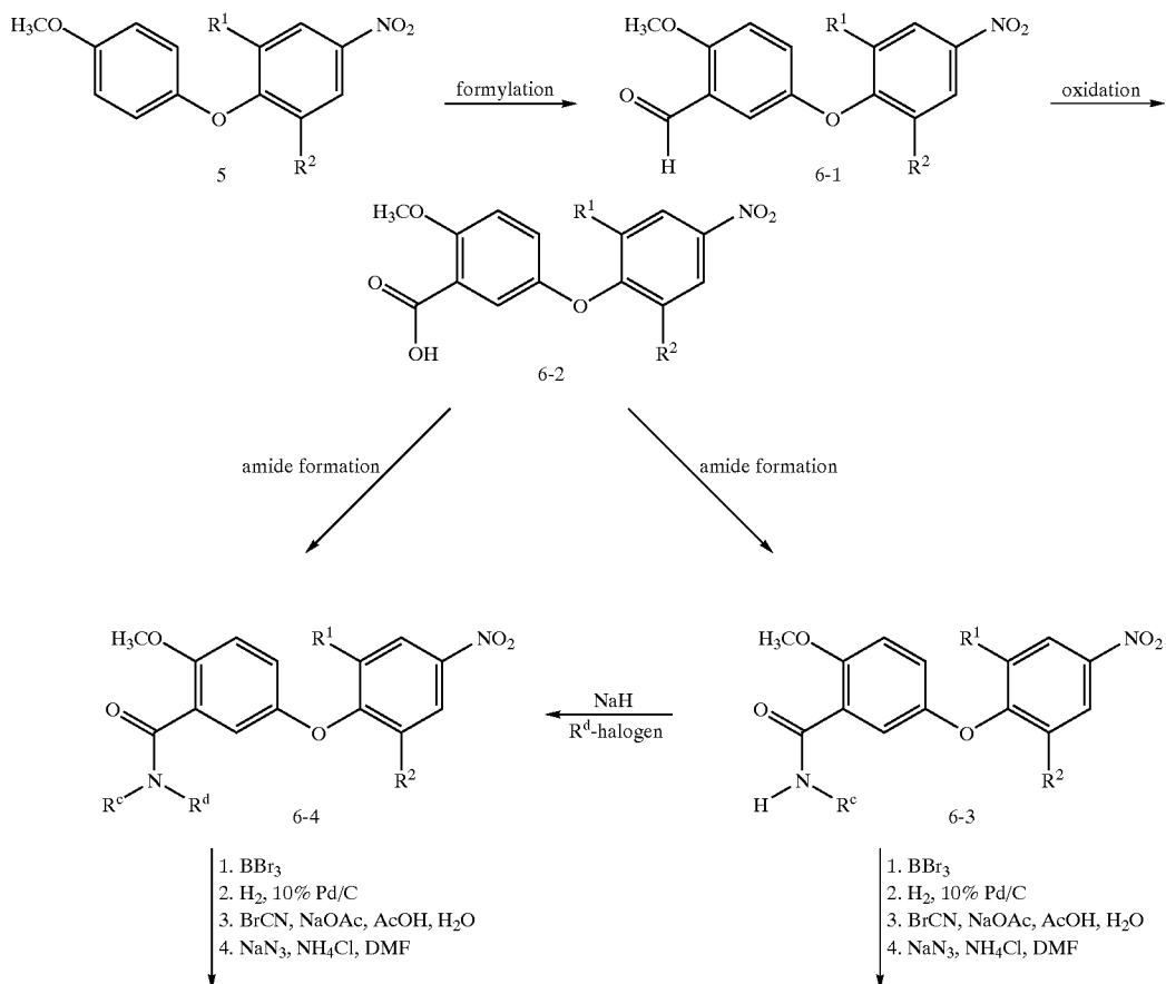
Scheme 6
