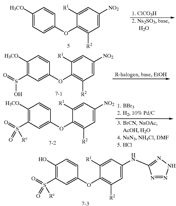
Scheme 8
