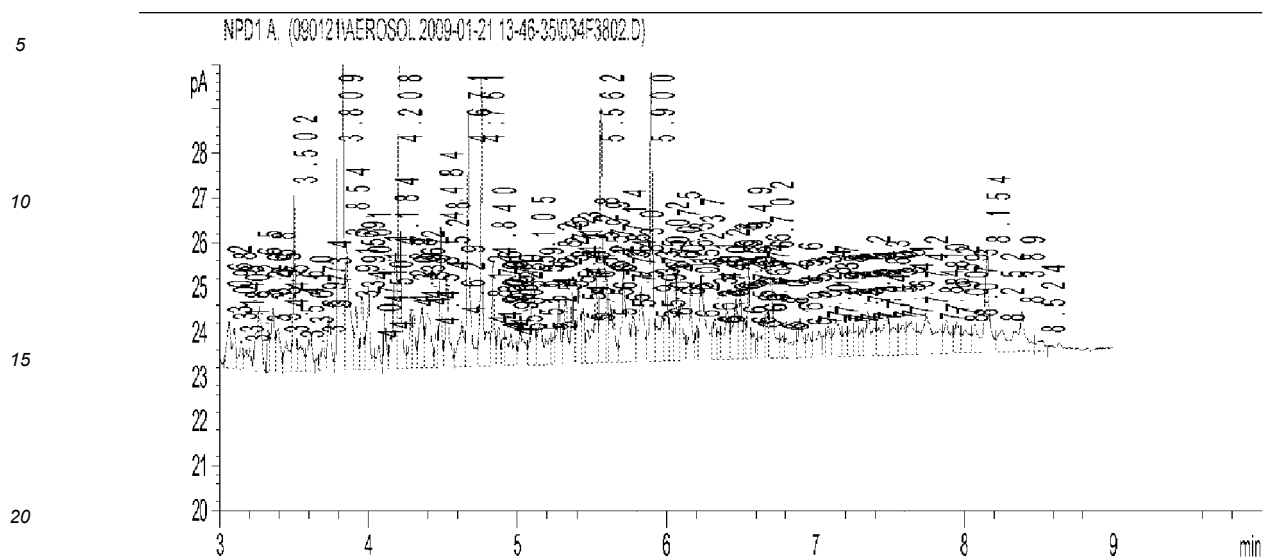
Picture 5. Total Ion Chromatogram of Marlboro Cigarette Extract
