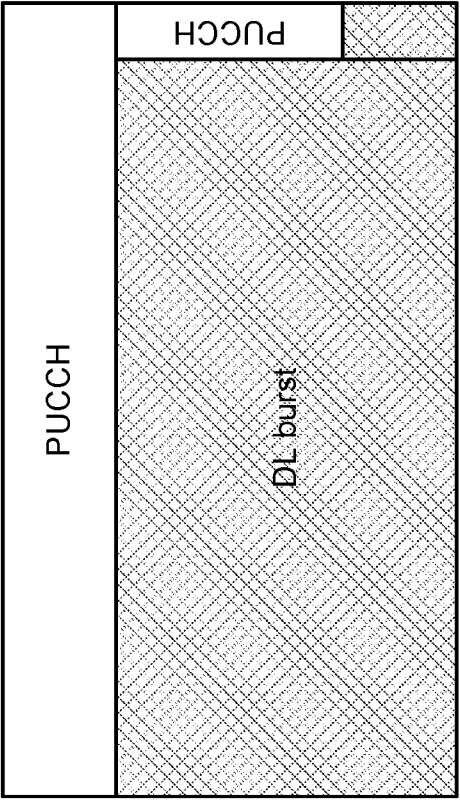
TDD UL only slot
