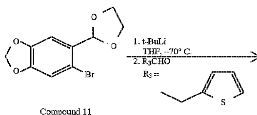
Reaction Scheme 1A
