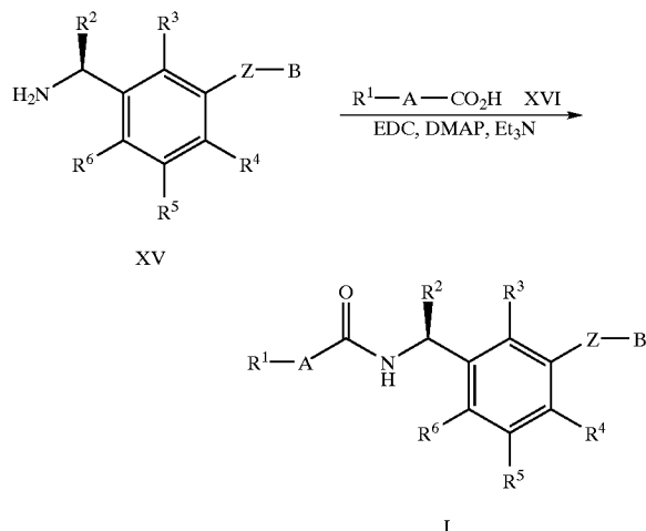
Reaction Scheme 5
