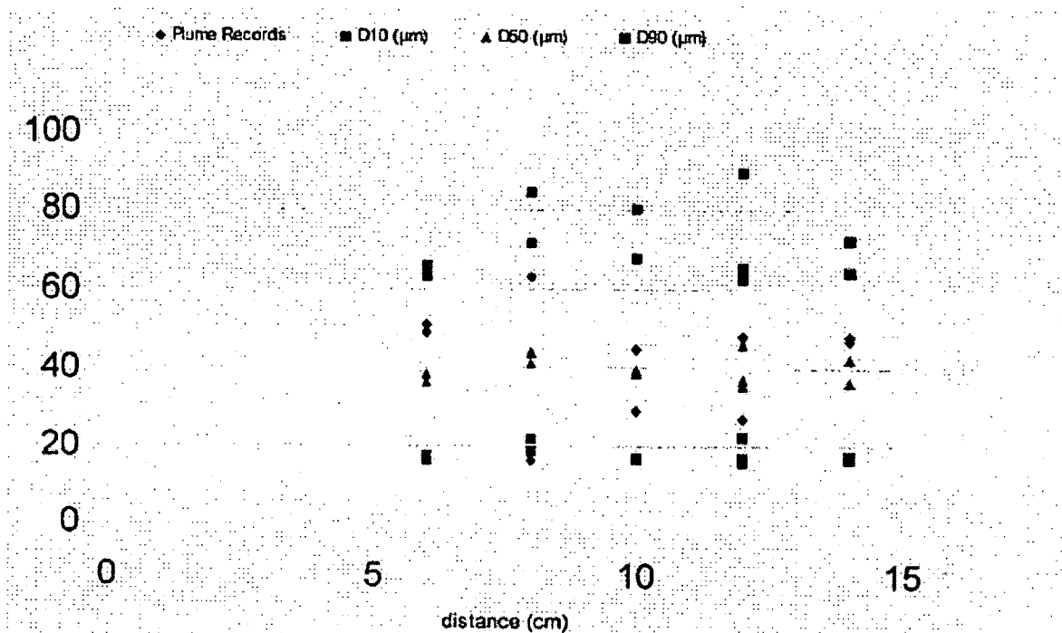
Figure 11: Vignetting Results Dv10, Dv50, Dv90 vs. Distance from Range Lens
