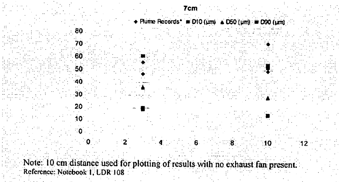
Figure 13: Exhaust Results Dv10, Dv50, Dv90 vs. Distance to Exhaust at 7 cm Device to Laser Beam
