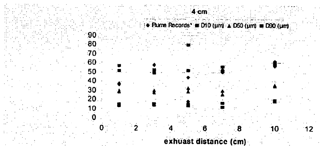
Figure 12: Exhaust Results Dv10, Dv50, Dv90 vs. Distance to Exhaust at 4 cm Device to Laser Beam
