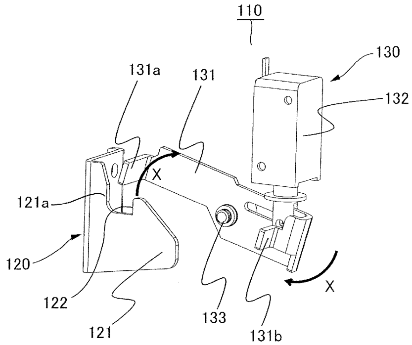
UNLOCK STATE
