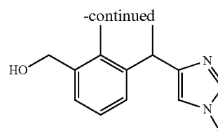
(3-(1-(1H-imidazol-4-yl)ethyl)- 2-methylphenyl)methanol
