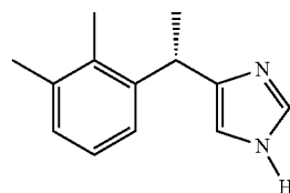
Dexmedetomidine (S)-4-[1-(2,3-dimethylphenyl) ethyl]-1H-imidazole CAS 189255-79-6
