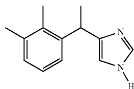
Medetomidine 4-[1-(2,3-dimethylphenyl) ethyl]-1H-imidazole CAS 86347-14-0
