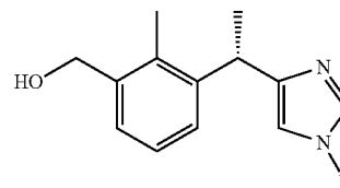
(S)-[3-(1-(1H-imidazol-4-yl)ethyl)- 2-methylphenyl)methanol
