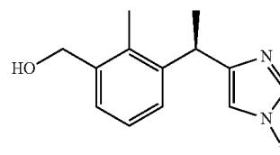
(R)-[3-(1-(1H-imidazol-4-yl)ethyl)- 2-methylphenyl)methanol
