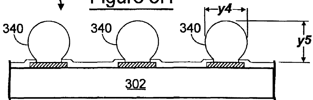
300 Figure 3H
