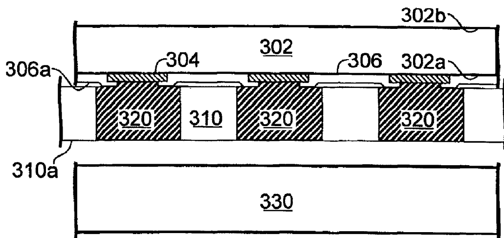
300 Figure 3F
