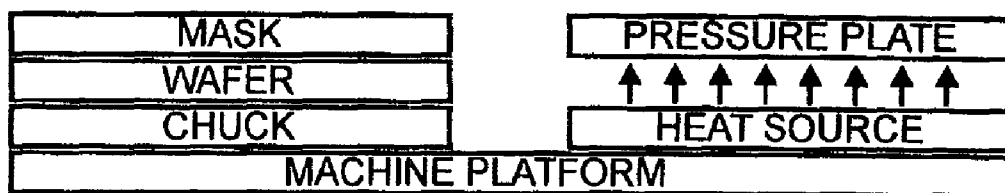
420 → Figure 4A
