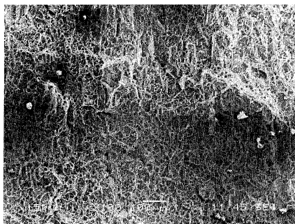
Fractography of A sample tested at -65F (showing ductile fracture mode)
