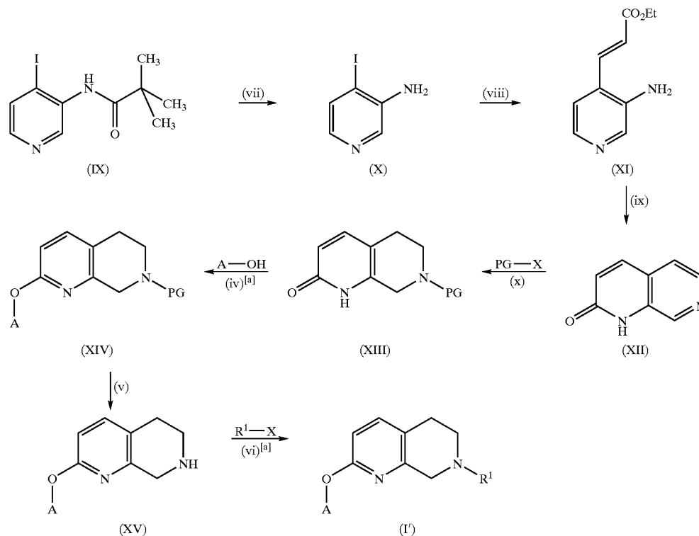
Scheme 2
