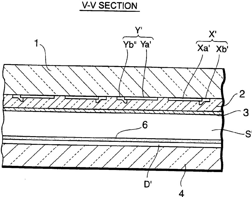
Fig.49 (PRIOR ART)
