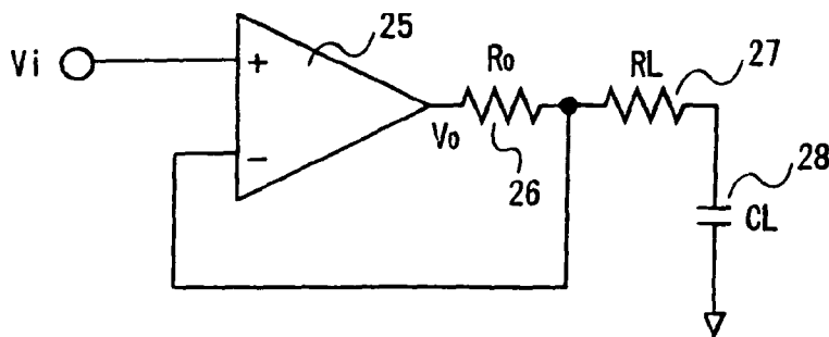
FIG. 7 RELATED ART
