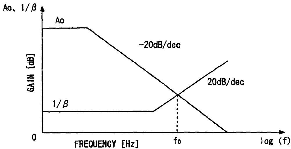
FIG. 6 RELATED ART
